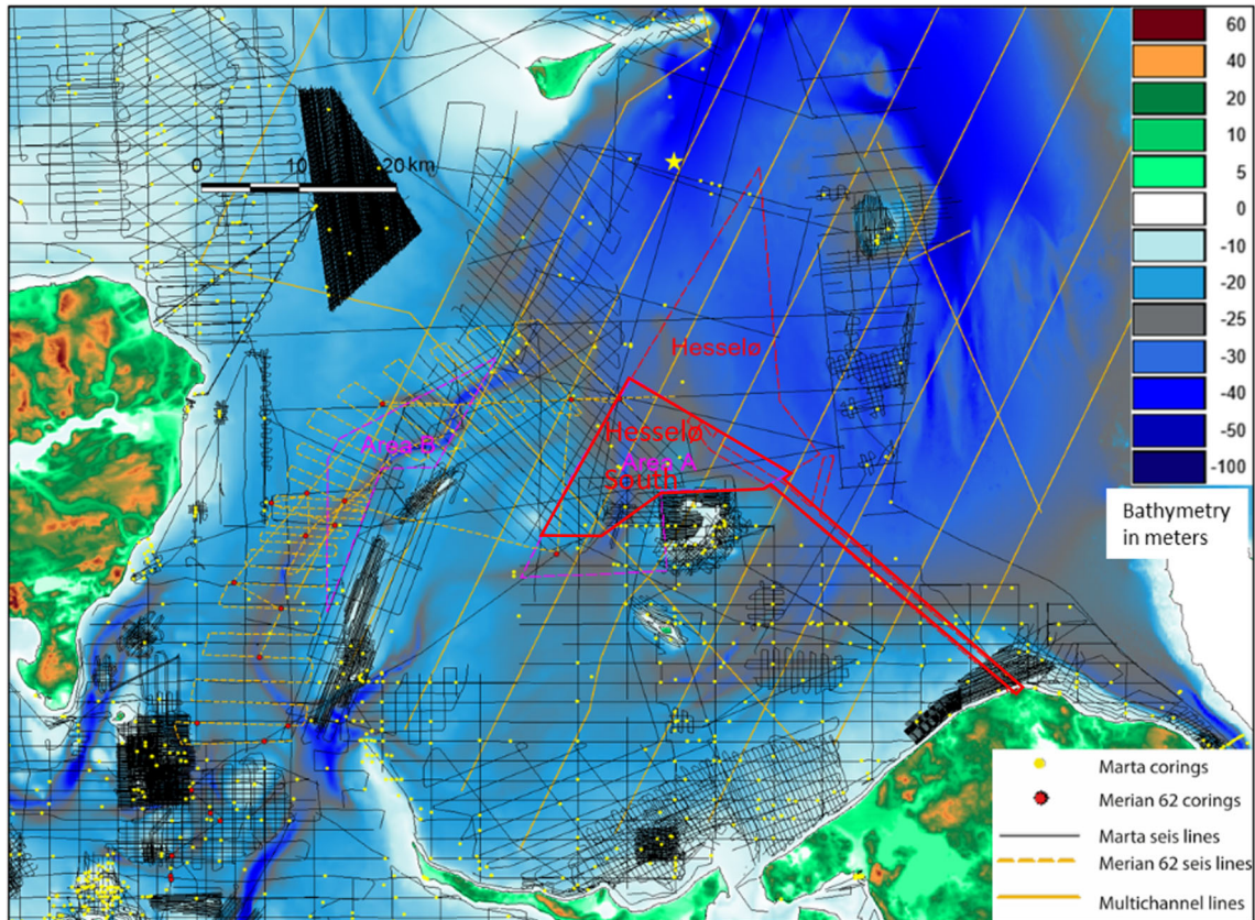
Figure 4.1. Distribution of Marta database seismic grid and core data in the southern and central Kattegat region. The Hesselø South OWF area and cable route is shown with red together with the existing Anholt OWF and OWF areas covered in previous screening reports (purple and red hatched lines). Bathymetry from www.emodnet-bathymetry.eu .
