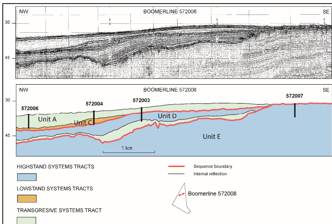
Figure 6.2. Boomer seismic section 572008.
