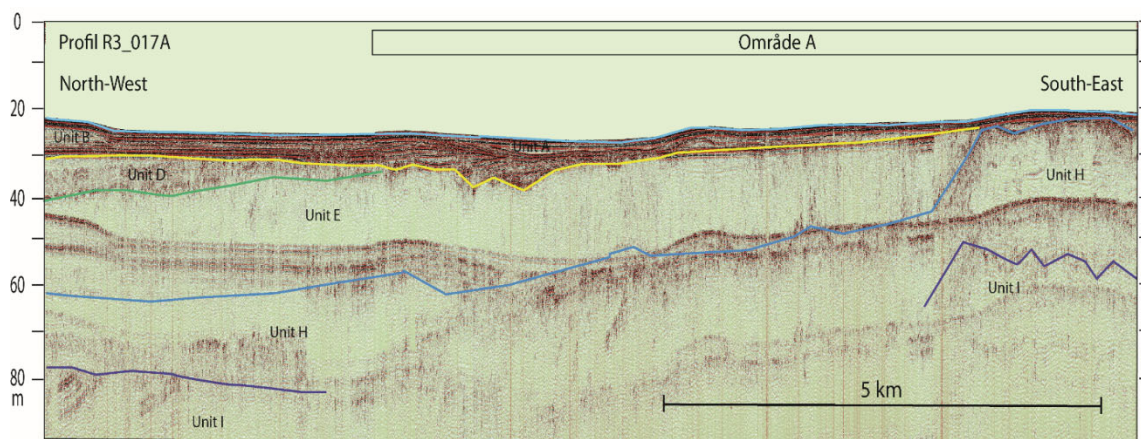
Figure 9.3 Northwest to southeast section through the Hesselø South OWF area. For location see Figure 9.1. The seismostratigraphic units are shown in Table 1.
