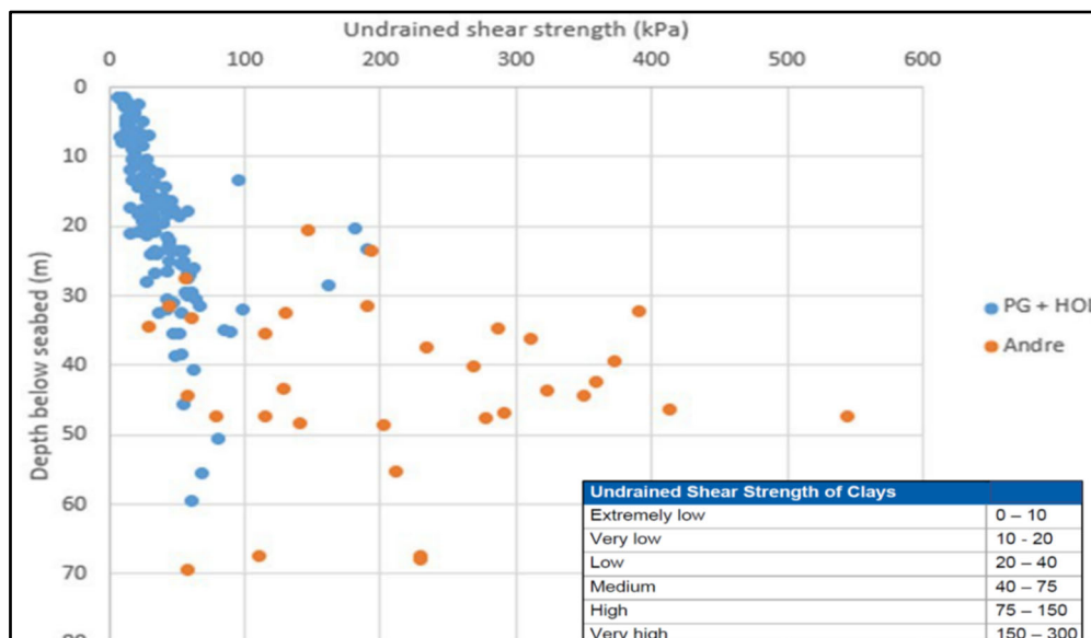
Figure 7.2 Undrained shear stress measurements showing low Unit A - E/F values and higher values for the lower units G–H.
