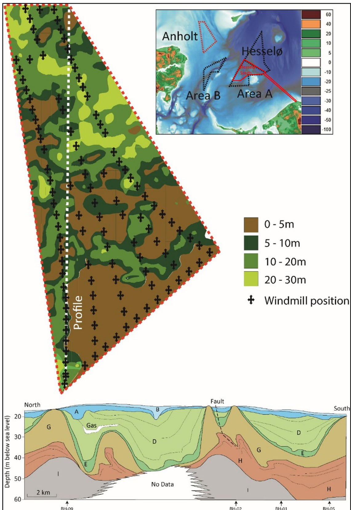
Figure 10.1 Anholt OWF general map of thickness of geotechnical soft sediment, with indication of location of schematic profile and windmill positions. Details of seismic units A–I in the schematic profile are provided in Table 1.
