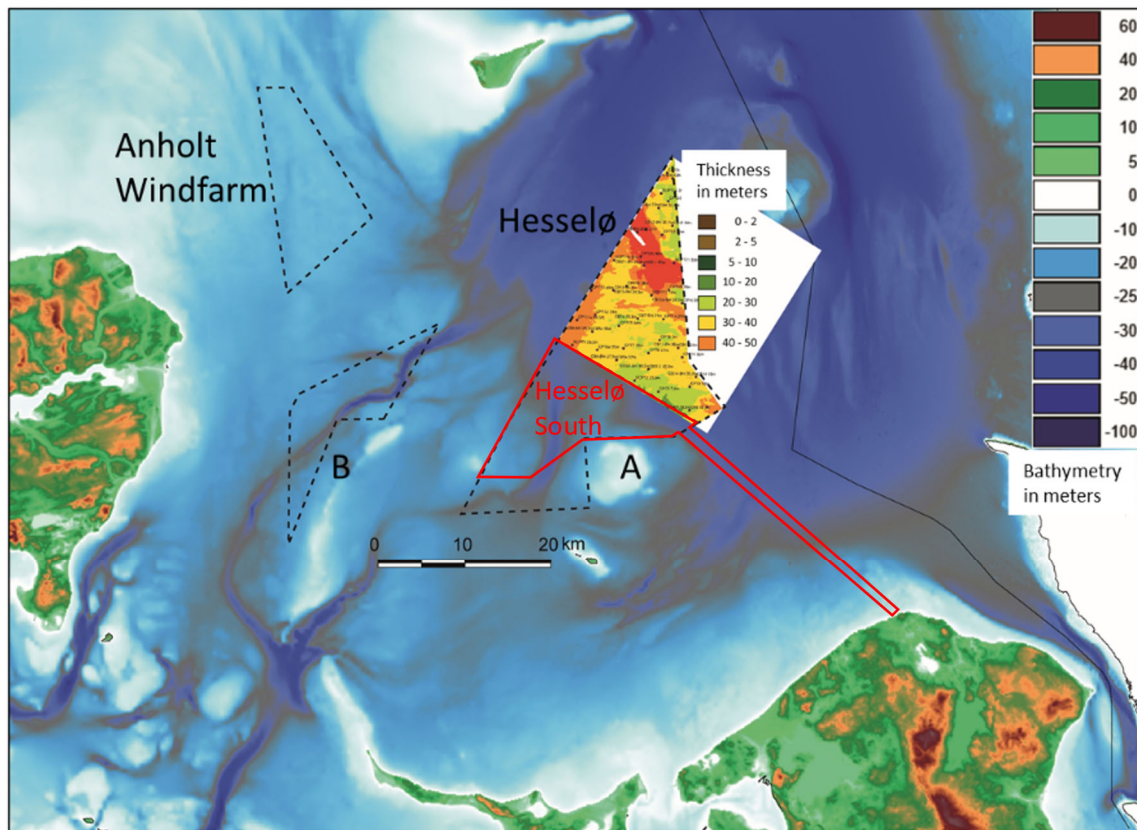
Figure 8.1 Detailed mapping of geotechnical soft sediments in the previous Hesselø OWF area. The Hesselø South OWF area and cable route is shown with red together with the existing Anholt OWF and OWF areas covered in previous screening reports (black hatched lines).
