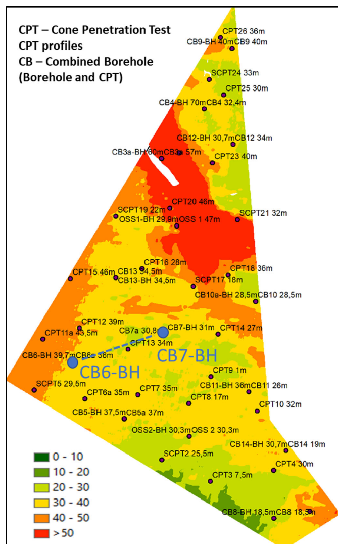
Figure 7.3 Thickness of geotechnical soft sediments (combined thickness of seismic Units A–E/F) in the previous Hesselø OWF area. Point data show thickness of soft sediments (CPT and boreholes). There is generally a good correlation between the data sets. Local areas without correlation could be related to glacial disturbance of Unit E/(F). Figure from Energinet (2021).
