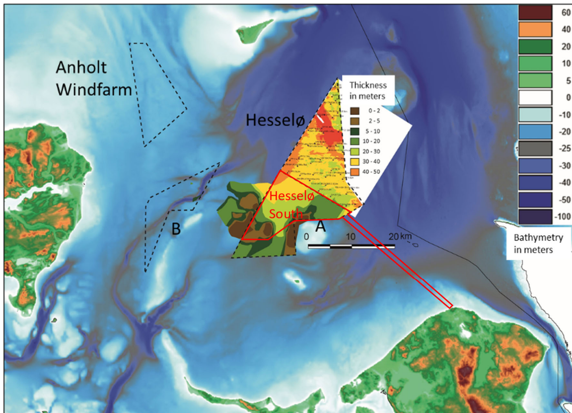
Figure 12.1 General thickness of geotechnical soft sediments (combined thickness of seismic Units A–E/F) in the current Hesselø South OWF area compared with the detailed mapping of the previous Hesselø OWF area. The Hesselø South OWF area and cable route is shown with red together with the existing Anholt OWF and OWF areas covered in previous screening reports (black hatched lines).
