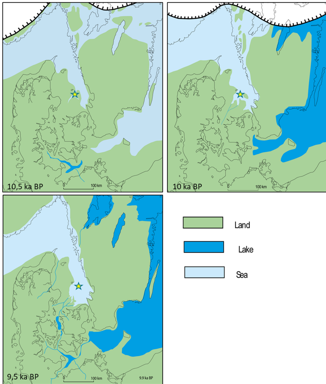
Figure 5.8. Palaeogeographical scenarios for the Kattegat region. There was a lowstand at 10.5 ka BP followed by a transgression (Jensen et al 2002). The yellow star shows the location of IODP core M0060.
