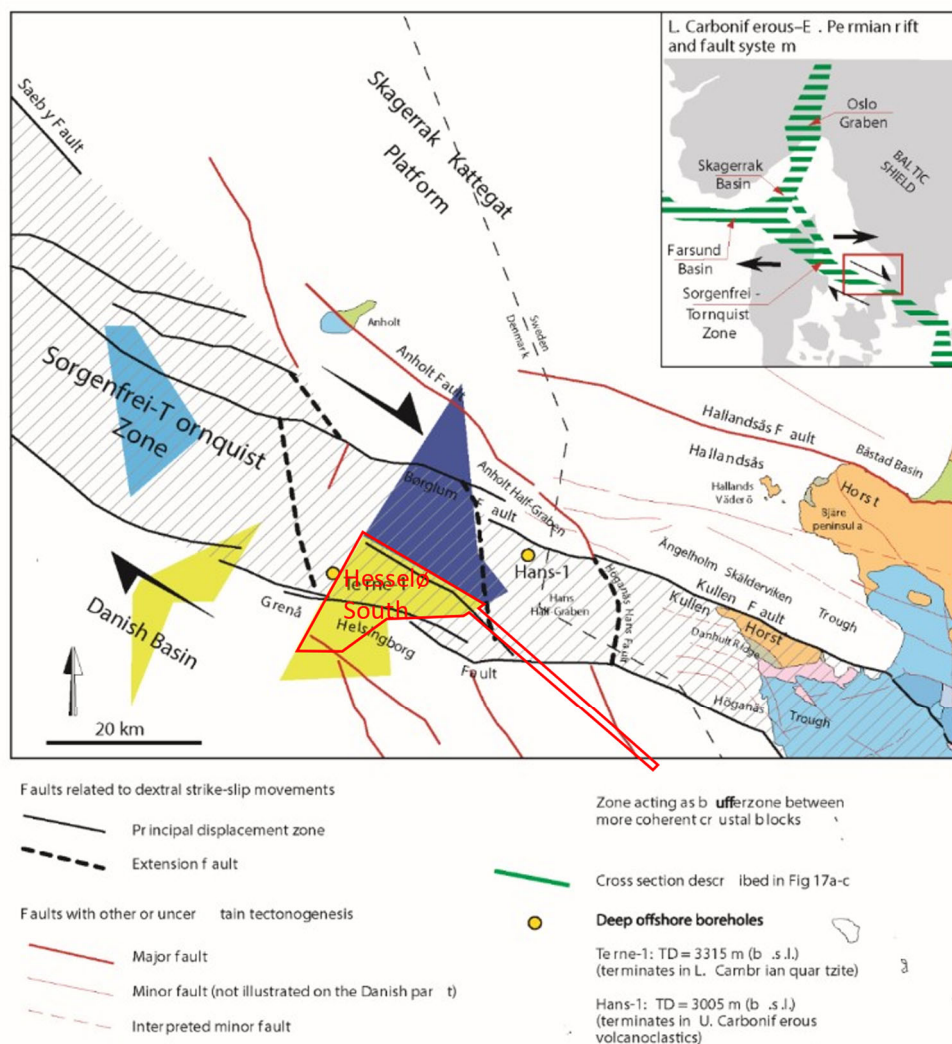
Figure 5.1. Regional structures in the southern part of the Kattegat (Erlström and Sivhed 2001). The location of the Hesselø South OWF area and cable route is shown in red together with the existing Anholt OWF (light blue) and OWF areas covered in previous screening reports (yellow and dark blue).
