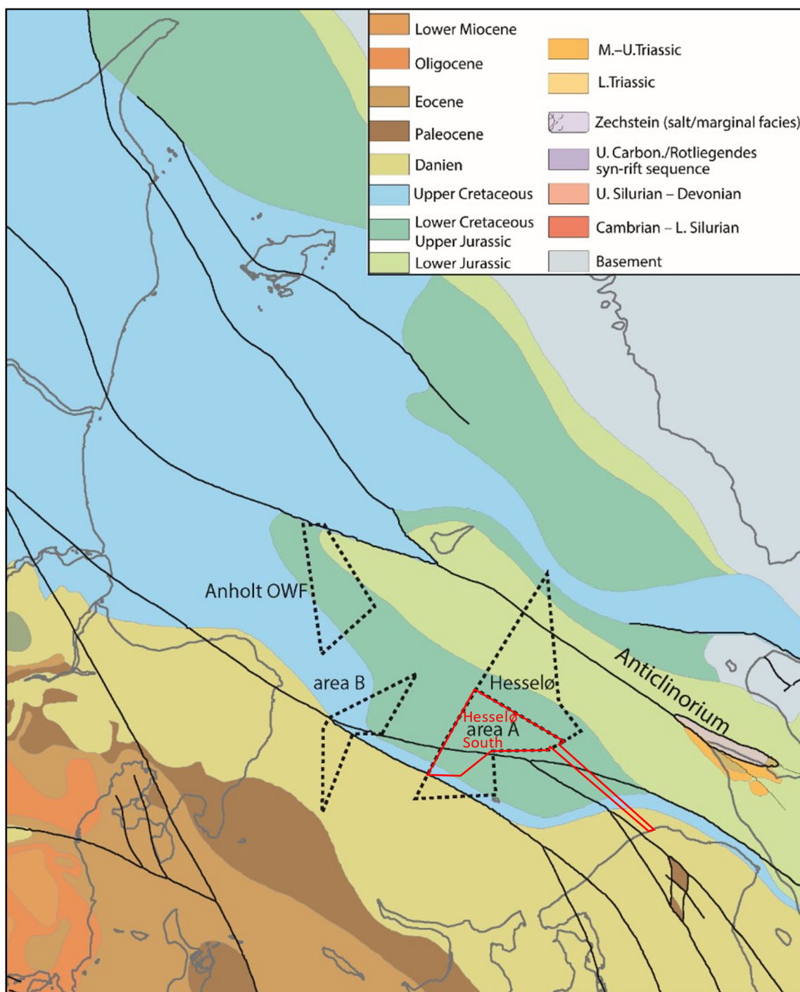
Figure 5.2. Pre-Quaternary surface geology and major faults in the Kattegat. The location of the Hesselø South OWF area and cable route is shown in red together with the existing Anholt OWF and OWF areas covered in previous screening reports (black hatched lines).
