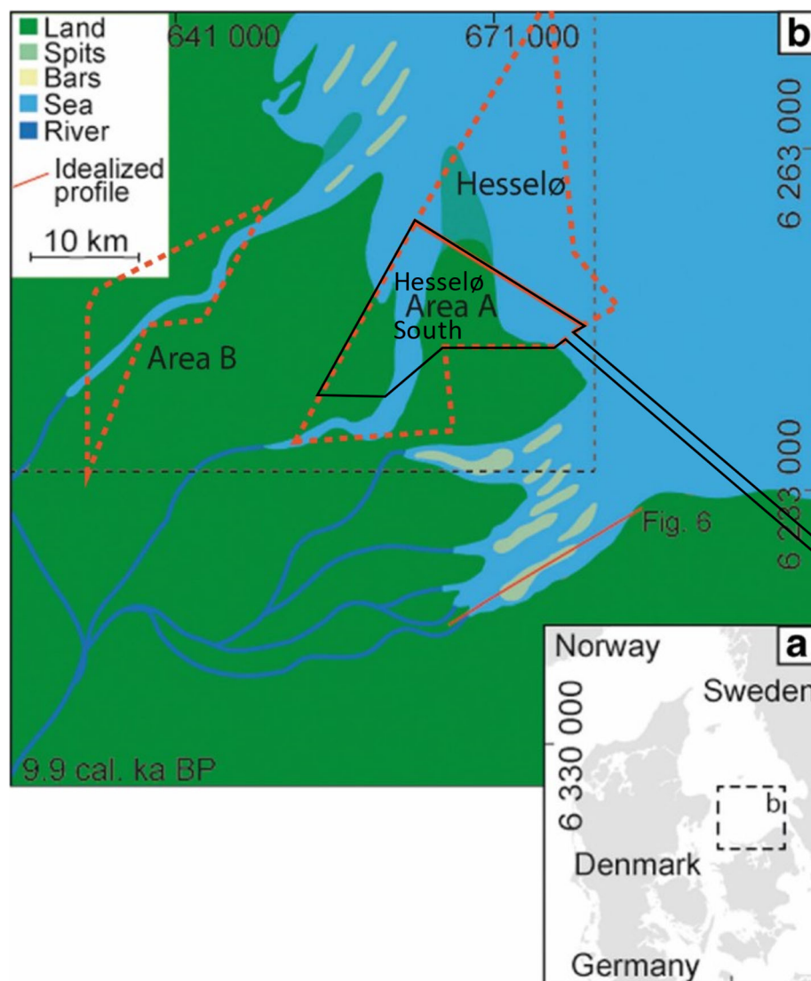
Figure 6.4 Dana River System Great Belt palaeo-river (Bendixen et al. 2015, 2017). The Hesselø South OWF area and cable route is shown with black together with the existing Anholt OWF and OWF areas covered in previous screening reports (red hatched lines).
