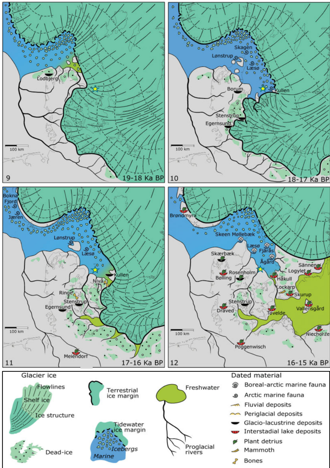
Figure 5.4. Palaeogeographical reconstructions of the last deglaciation of southern Scandinavia (19–15 ka BP; Houmark-Nielsen & Kjær 2003).
