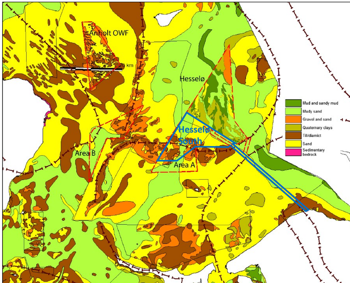
Figure 5.10. Seabed surface sediment map with interpreted ice marginal ridges. The Hesselø South OWF area and cable route is shown with blue together with the existing Anholt OWF and OWF areas covered in previous screening reports (red hatched lines). Updated detailed sediment data from Fugro (2021) is presented north of the Hesselø South OWF area and thin black lined polygons marks margins of detailed mapped subareas. Bathymetry from www.emodnet-bathymetry.eu .
