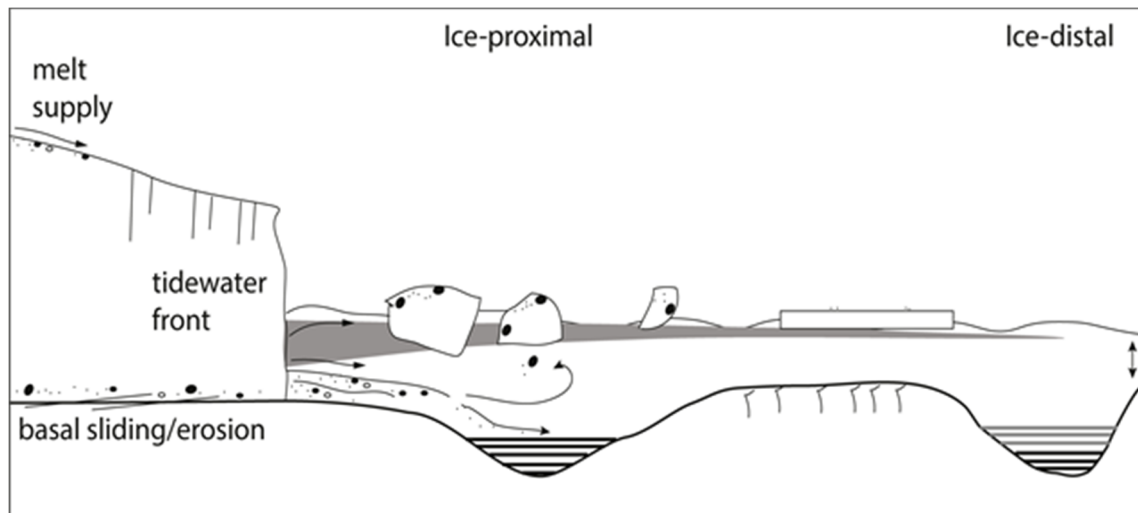
Figure 5.5. Illustration of a glaciomarine depositional environment.
