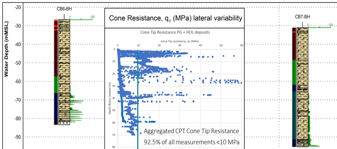
Figure 7.1 Geotechnical sediment cores CB6-BH and CB7-BH, with indication of very low cone resistance to more than 40 m below seabed and evidence of 92,5% of total CPT measurements below 10 MPa. The location of CB6-BH and CB7-BH is indicated on Figure 7.3.
