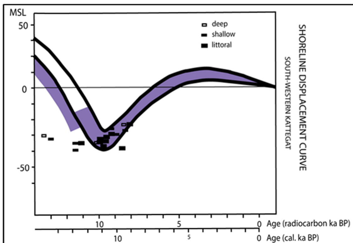
Figure 5.7. Shoreline displacement curves for the southern Kattegat. The two solid black lines indicate the range of shoreline displacements in non-faulted regions of the study area (modified from Mörner 1983). The purple area indicates the relative sea level changes interpreted from the sequence stratigraphy in the down-faulted NW–SE-striking depression. Radiocarbon dated samples are indicated as deep >10 m, shallow 2–10 m or littoral 0–2 m.
