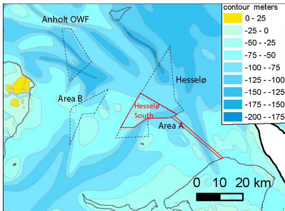
Figure 5.3. General pre-Quaternary morphology (Binzer & Stockmarr 1994). The location of the Hesselø South OWF area and cable route is shown in red together with the existing Anholt OWF and OWF areas covered in previous screening reports (black hatched lines).
