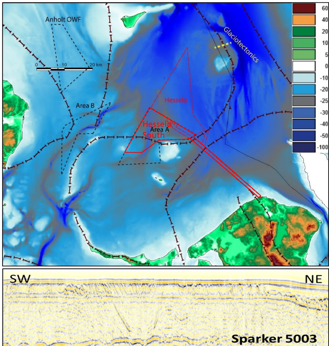
Figure 5.6. Upper figure: Interpreted ice marginal ridges in the southern part of the Kattegat. Lower figure: Sparker profiler showing evidence of glaciotectionic deformations north of Store Middelgrund (yellow dashed line on upper figure). The Hesselø South OWF area and cable route is shown with red together with the existing Anholt OWF and OWF areas covered in previous screening reports (black and red hatched lines). Bathymetry from www.emodnet-bathymetry.eu .
