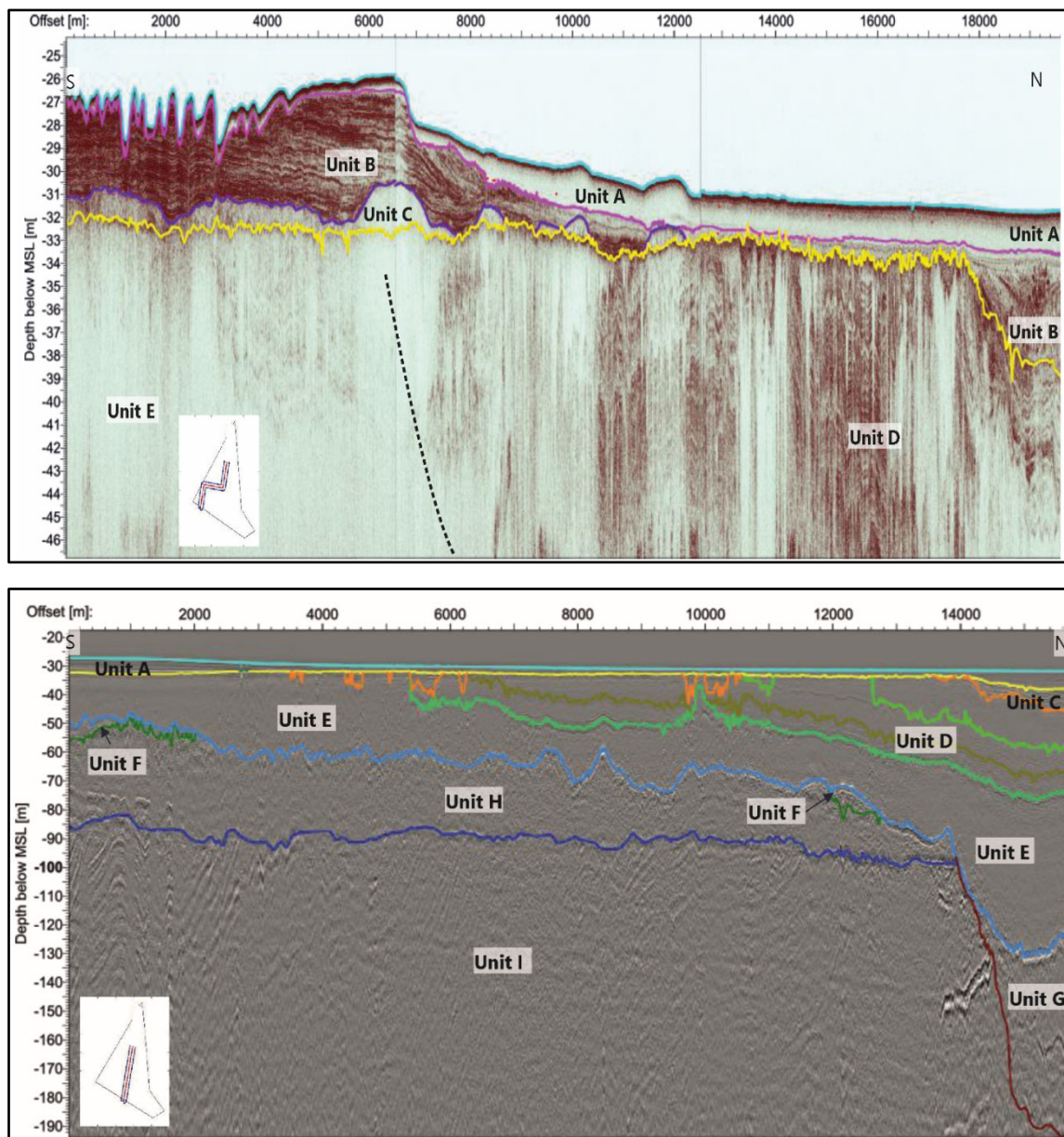
Figure 6.1. Overview of seismostratigraphic units interpreted in the previous Hesselø OWF study area.
