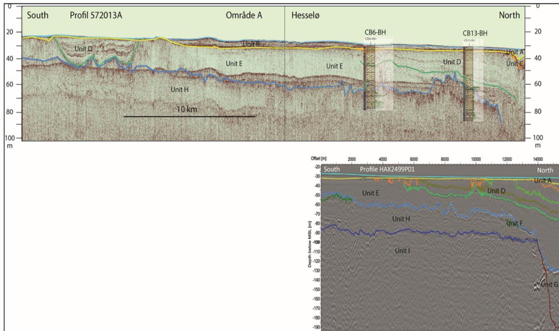
Figure 9.2 North-south seismic profiles Fugro line HAX2499P01 and archive line 572013A continuing southward from the previous Hesselø OWF area through the current Hesselø South OWF area. For location see Figure 9.1. The seismostratigraphic units are presented in Table 1.
