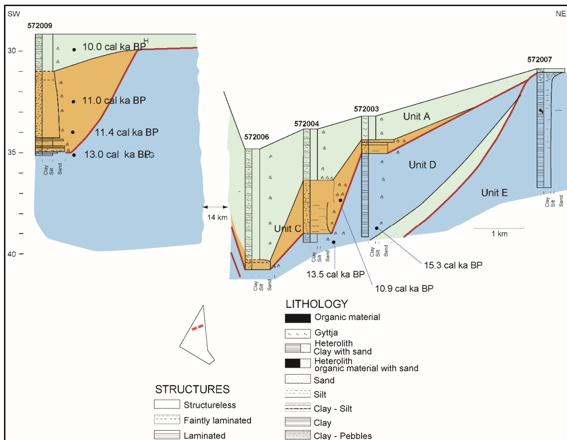
Figure 6.3. Sedimentological logs and log correlations. Sedimentological signatures are indicated; for description of stratigraphical signatures see Table 1. Overview of seismostratigraphic units adapted from GEUS (2020) and Fugro (2021). Detailed information on C-14 ages is given in Jensen et al. (2002).
