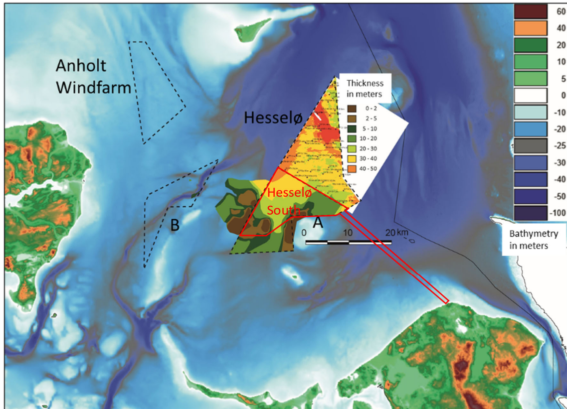
Figure 9.4 General thickness of geotechnical soft sediments (combined thickness of seismic Units A–E/F) in the current Hesselø South OWF area compared with the detailed mapping of the previous Hesselø OWF area. The Hesselø South OWF area and cable route is shown with red together with the existing Anholt OWF and OWF areas covered in previous screening reports (black hatched lines).
