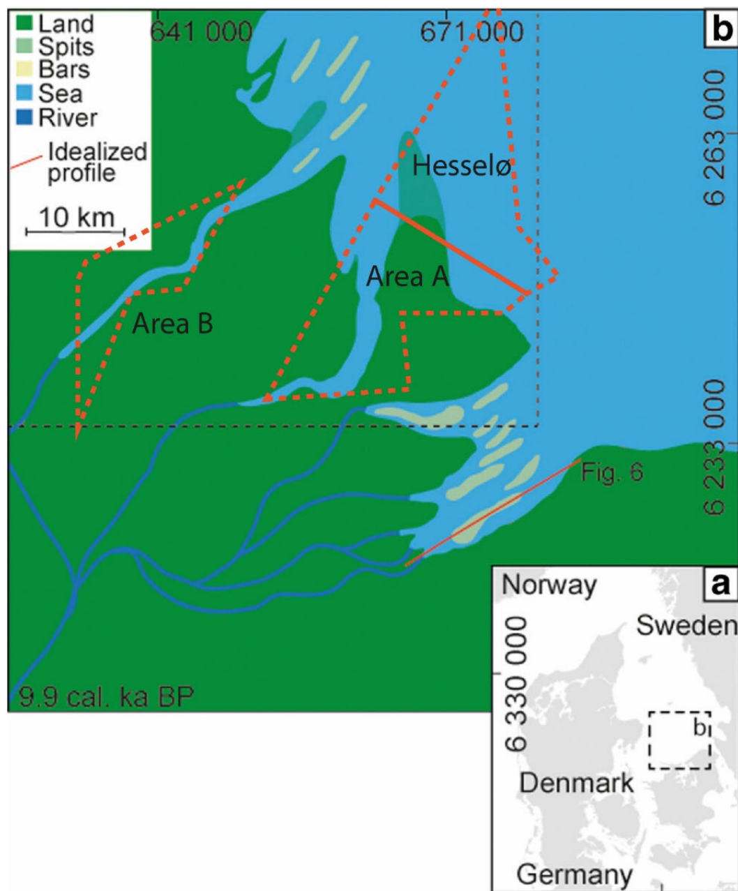
Figure 6.4 Dana River System Great Belt palaeo-river (Bendixen et al. 2015, 2017)
