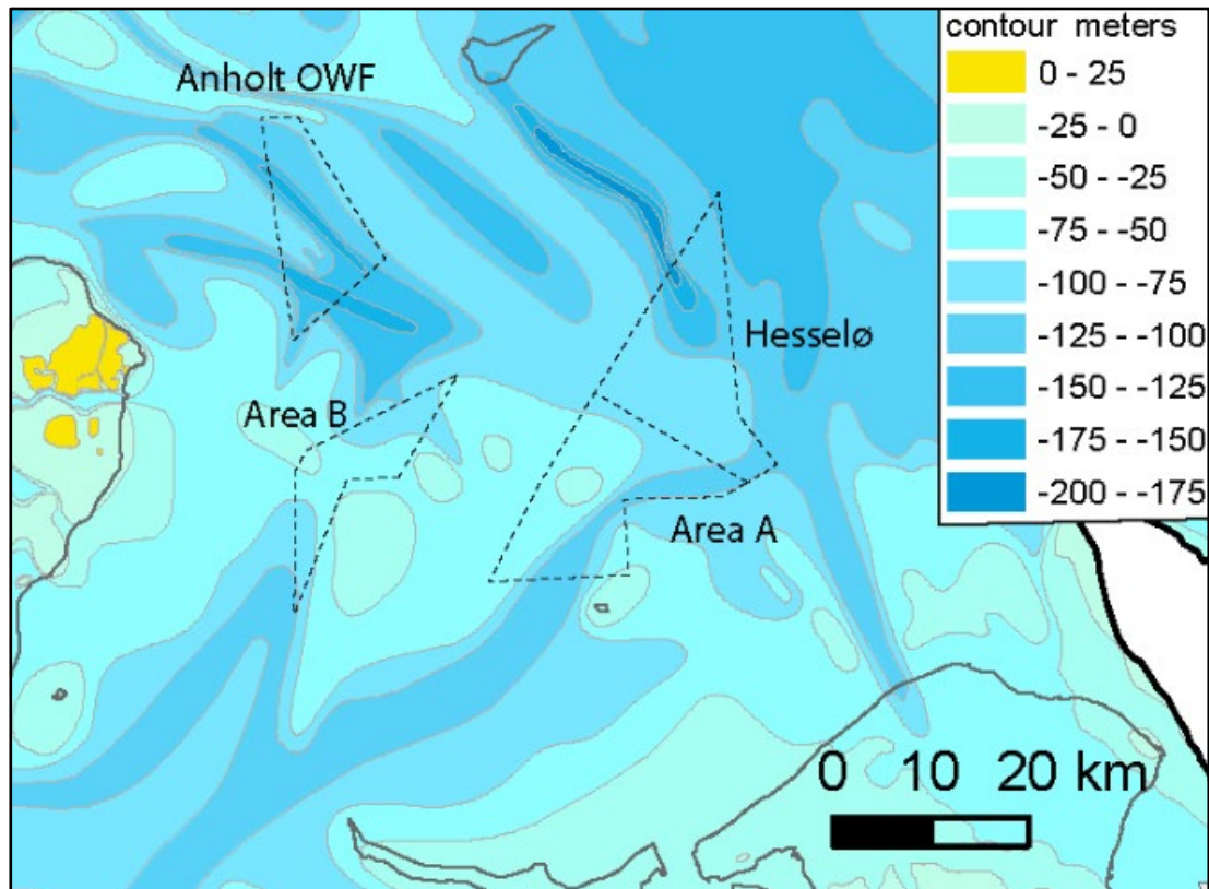
Figure 5.3. General pre-Quaternary morphology (Binzer & Stockmarr 1994). The location of the OWF's is indicated.
