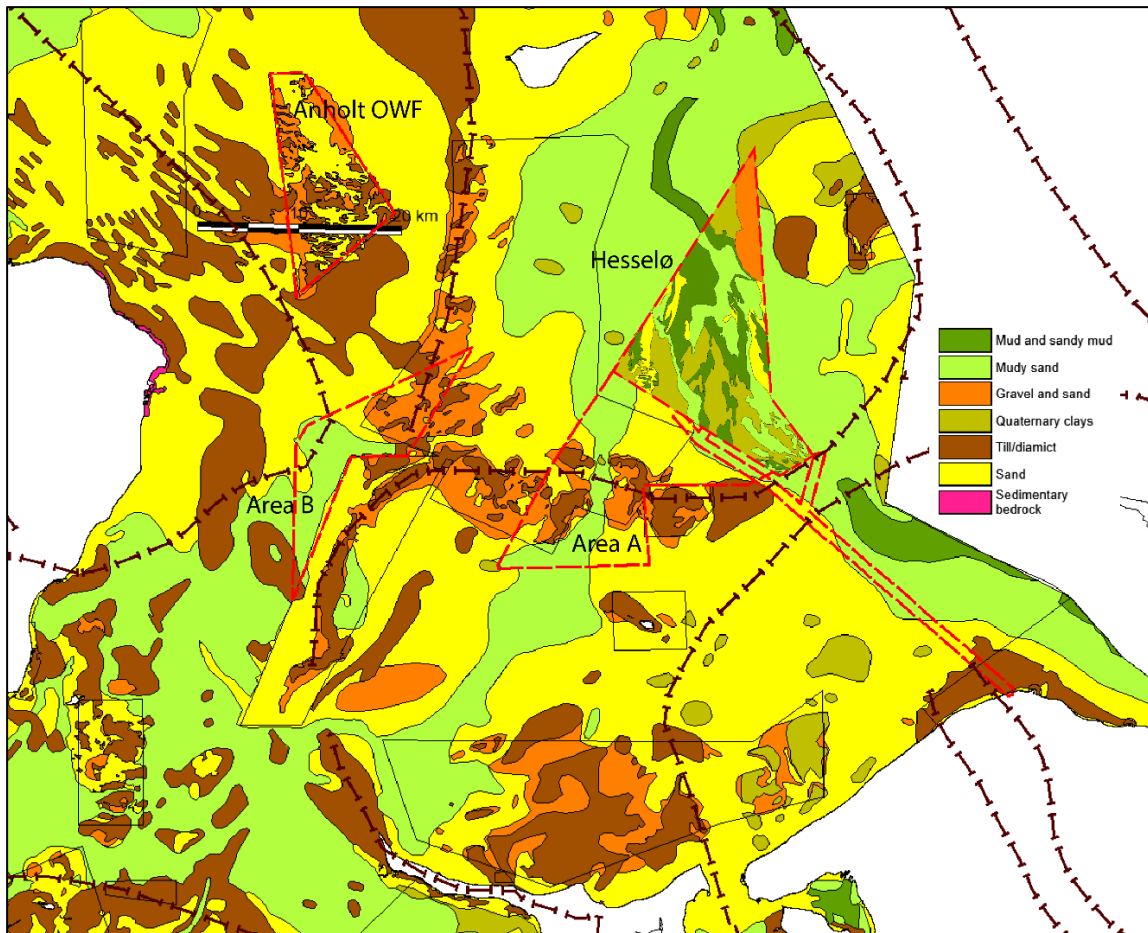
Figure 5.10. Seabed surface sediment map, interpreted ice marginal ridges. The locations of the existing Anholt OWF, the planned Hesselø OWF and the potential OWF areas A and B in the southern part of the Kattegat are indicated (red stippled polygons). Updated detailed sediment data from Fugro (2021) is presented in Hesselø OWF. (Black lined polygons marks margins of detailed mapped subareas).
