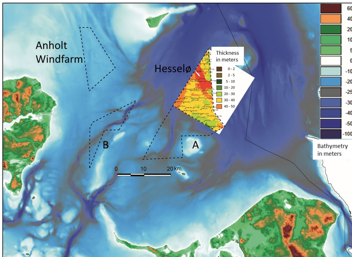
Figure 8.1 Detailed mapping of geotechnical soft sediments in Hesselø OWF, presented in relation to the optional study areas A and B as well as the existing Anholt OWF.
