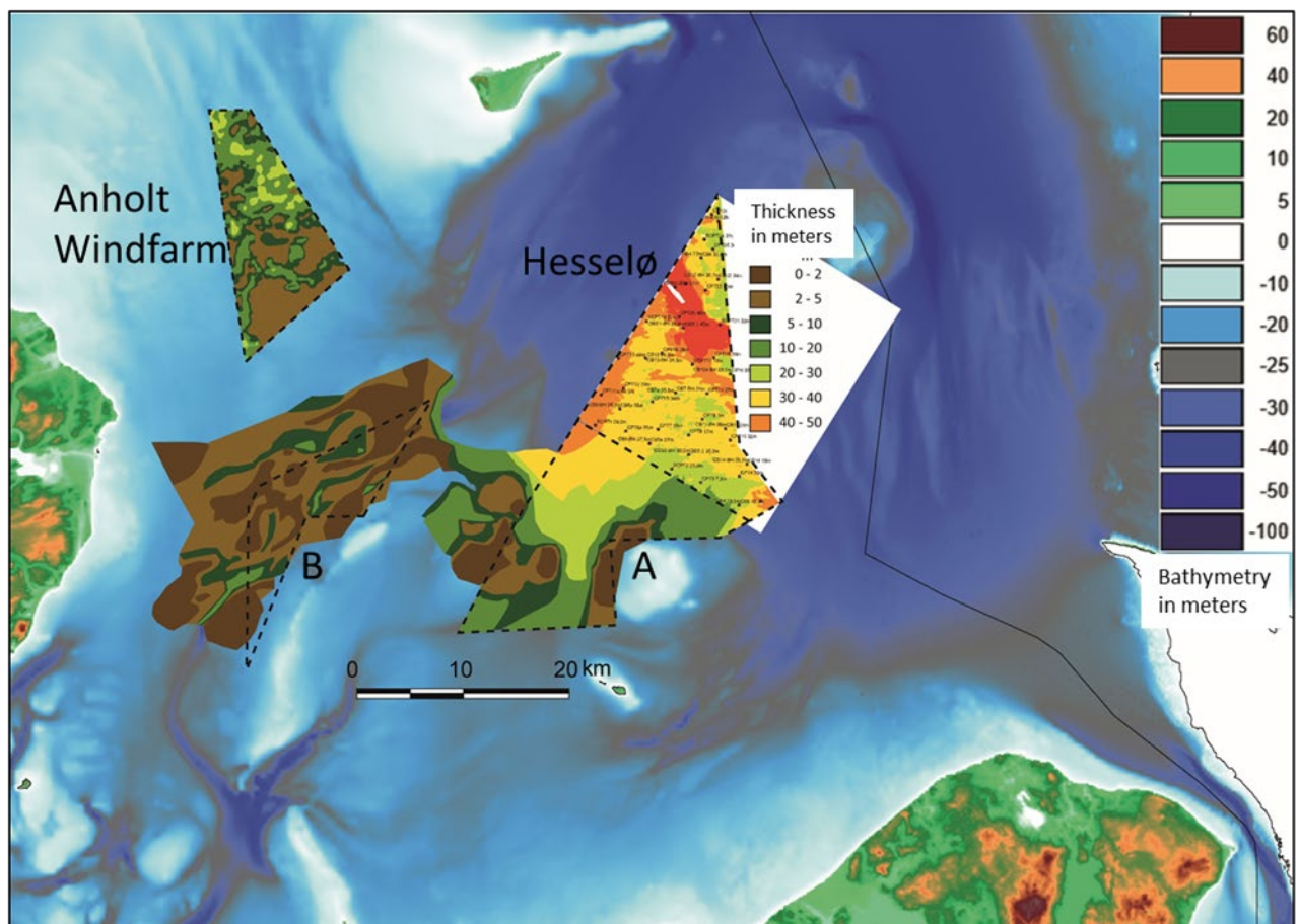
Figure 1.1 Thickness of geotechnical soft sediments in the southern Kattegat Anholt OWF and potential Hesselø, Area A and B. For details see Appendix C.
