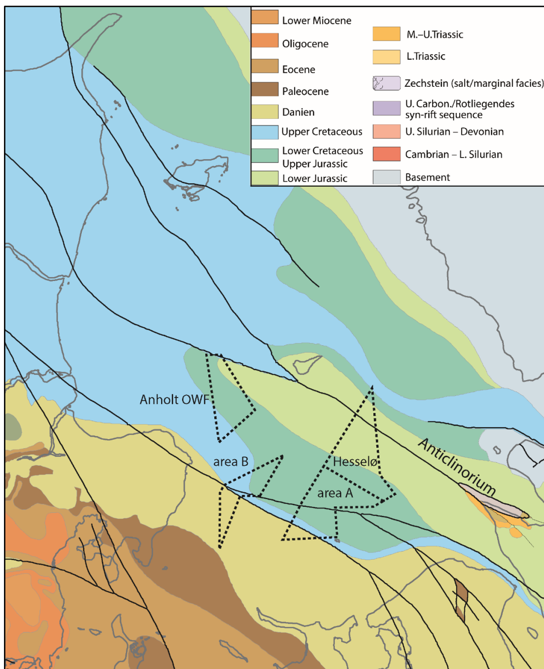
Figure 5.2. Pre-Quaternary surface geology and major faults in the Kattegat. The locations of the OWF's are indicated.
