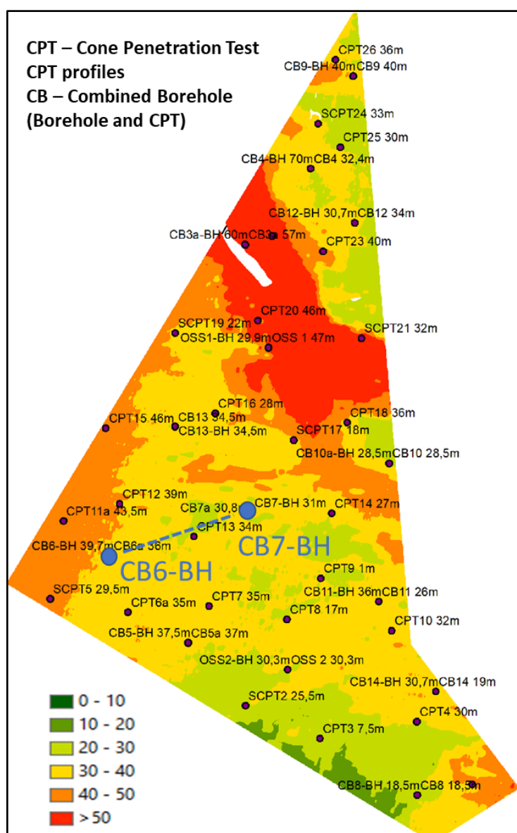
Figure 7.3 Thickness of geotechnical soft sediments (thickness of Unit A–E/F Seismic data) in the Hesselø OWF. Point data shows thickness of soft sediment (CPT and boreholes). There is generally a good correlation between the data sets. Local areas without correlation could be related to glacial disturbance of Unit E(F). Figure from Energinet (2021).
