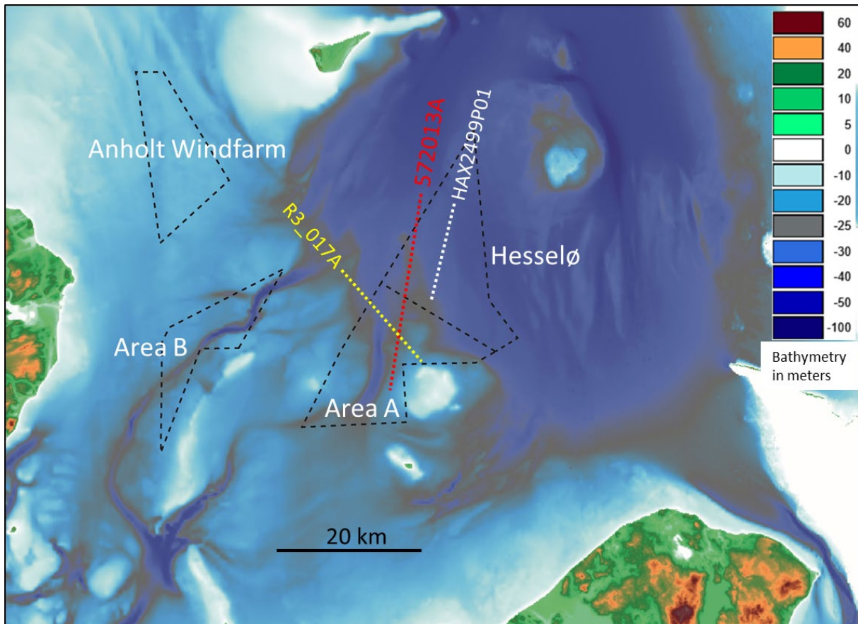
Figure 9.1 Bathymetry and location of seismic examples from Hesselø OWF and Area A.
