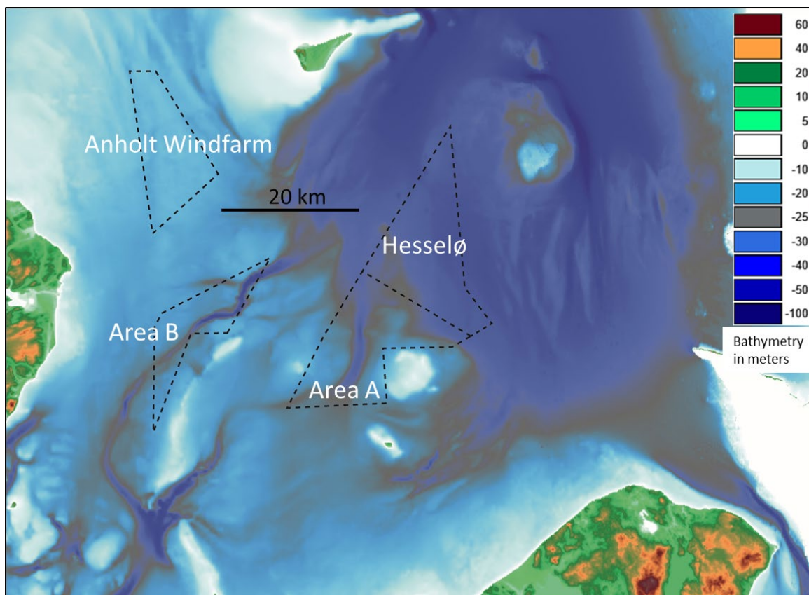
Figure 5.9 Southern Kattegat bathymetry. The locations of the existing Anholt OWF, the planned Hesselø OWF and the potential OWF areas A and B in the southern part of the Kattegat are indicated. Bathymetry from www.emodnet-bathymetry.eu .
