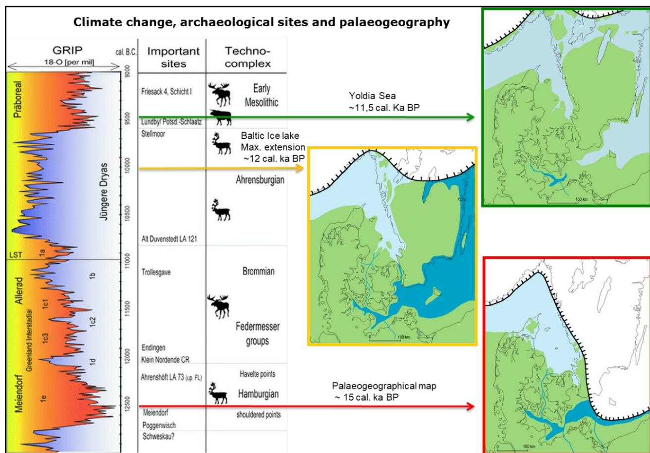
Figure 12.1. Late Glacial and Holocene general palaeogeography in Kattegat and related archaeological cultures. (the maps are from Jensen et al. 2003).
