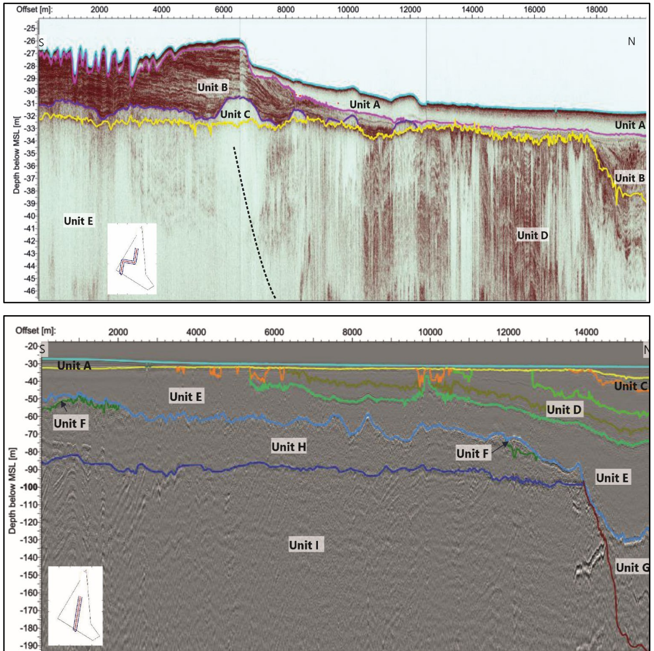
Figure 6.1. Overview of seismostratigraphic units interpreted in the Hesselø OWF study area.
