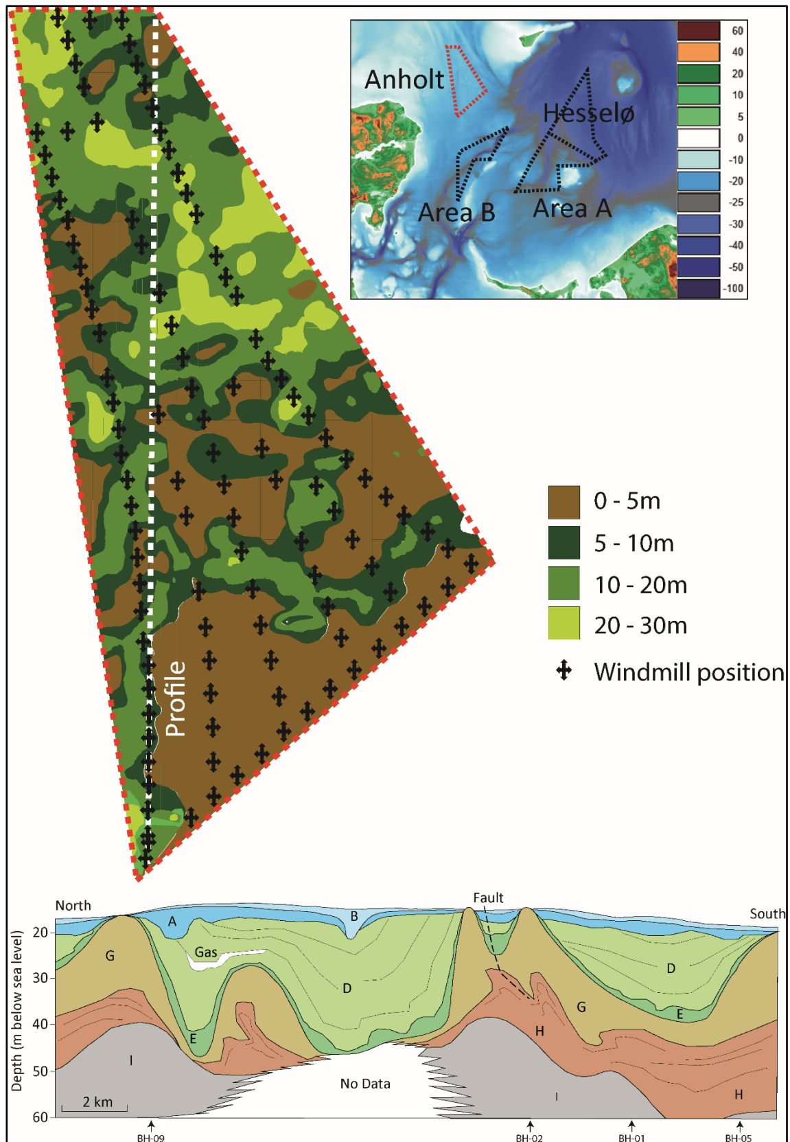
Figure 11.1 Anholt OWF general map of thickness of geotechnical soft sediment, with indication of location of schematic profile and windmill positions. Details of seismic units A–I in the schematic profile are provided in Table 1.
