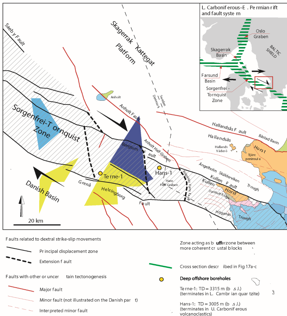
Figure 5.1. Regional structures in the southern part of the Kattegat (Erlström and Sivhed 2001). The locations of the existing Anholt OWF (light blue), the planned Hesselø OWF (dark blue) as well as the potential OWF areas A and B (yellow) are indicated.
