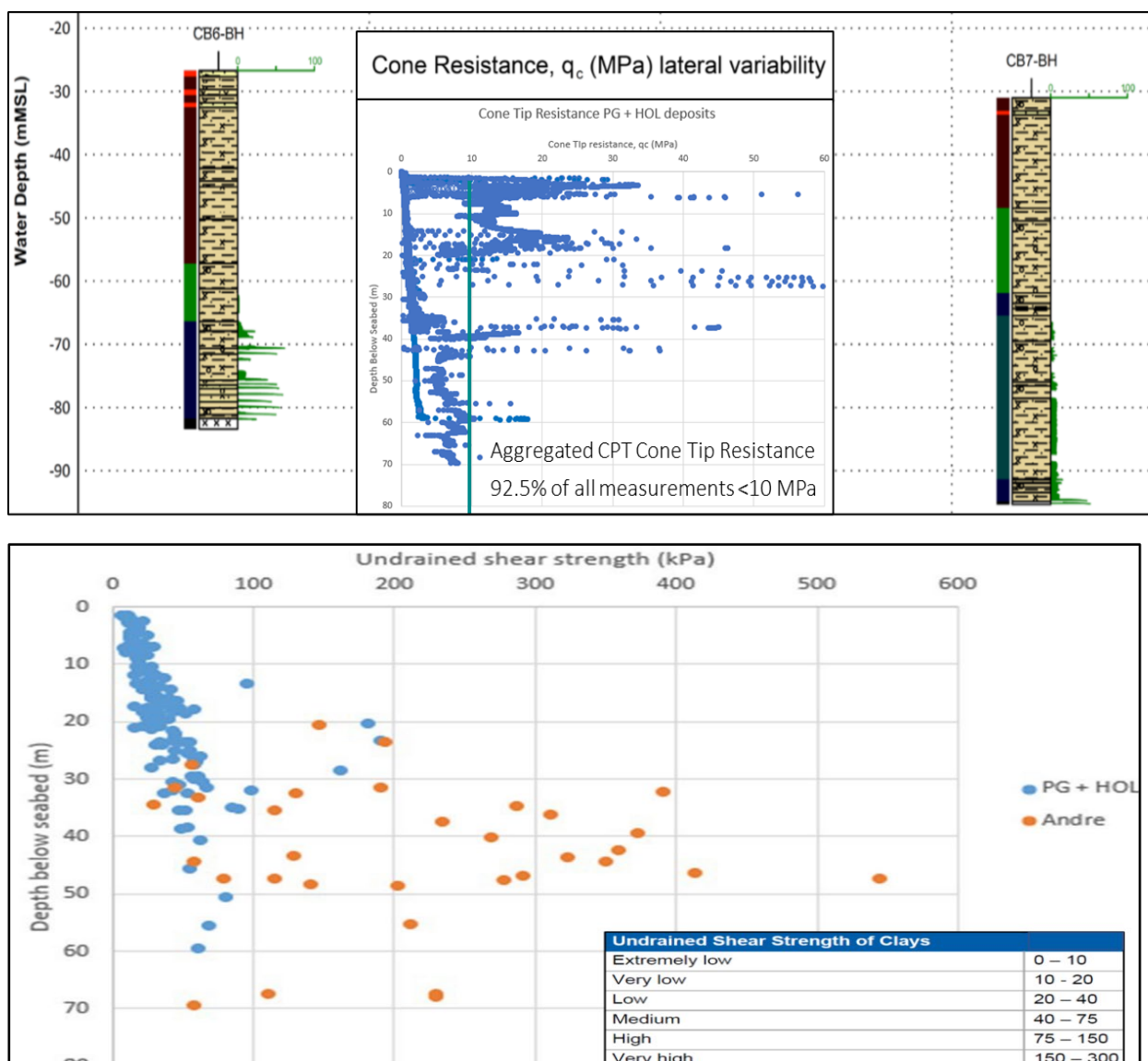
Figure 7.1 Geotechnical sediment cores CB6-BH and CB7-BH, with indication of very low cone resistance to more than 40 m below seabed and evidence of 92,5% of total CPT measurements <10 MPa. The location of CB6-BH and CB7-BH is indicated on Figure 7.3.
