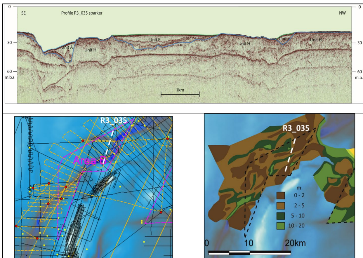
Figure 10.1 South-east to north-west Sparker profile R3_035 with documentation for location in relation to the seismic archive data grid and the geotechnical soft sediment thickness map.
