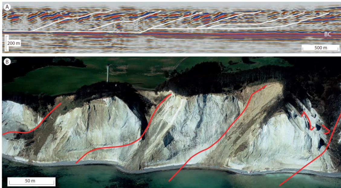
Figure 2.15. A comparison of thrust-fault architecture in two glaciotectionic complexes: A: Seismic section from the Jammerbugt Glaciotectionic Complex. See also Figure 2.13. B: The Møns Klint Glaciotectionic Complex. From Pedersen & Boldreel (2015).
