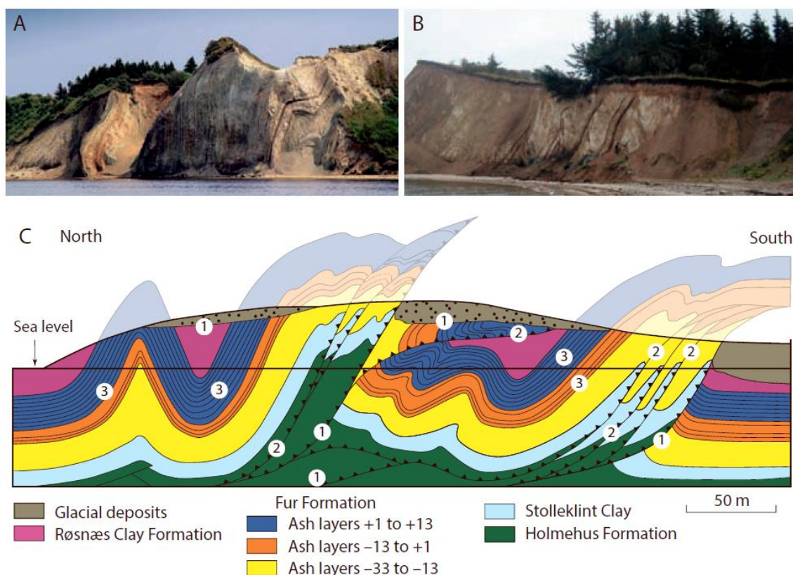
Figure 2.11. The Fur Knudeklint Glaciotectionic Complex. The Norwegian Ice Advance in the Late Weichselian deformed the Palaeogene clay formations. A and B: Photos from the cliff section: An anticline, a syncline, steeply dipping layers and imbricate duplexes. C: Schematic section. From Pedersen & Boldreel (2015). For further explanation, see Pedersen & Boldreel (2015).
