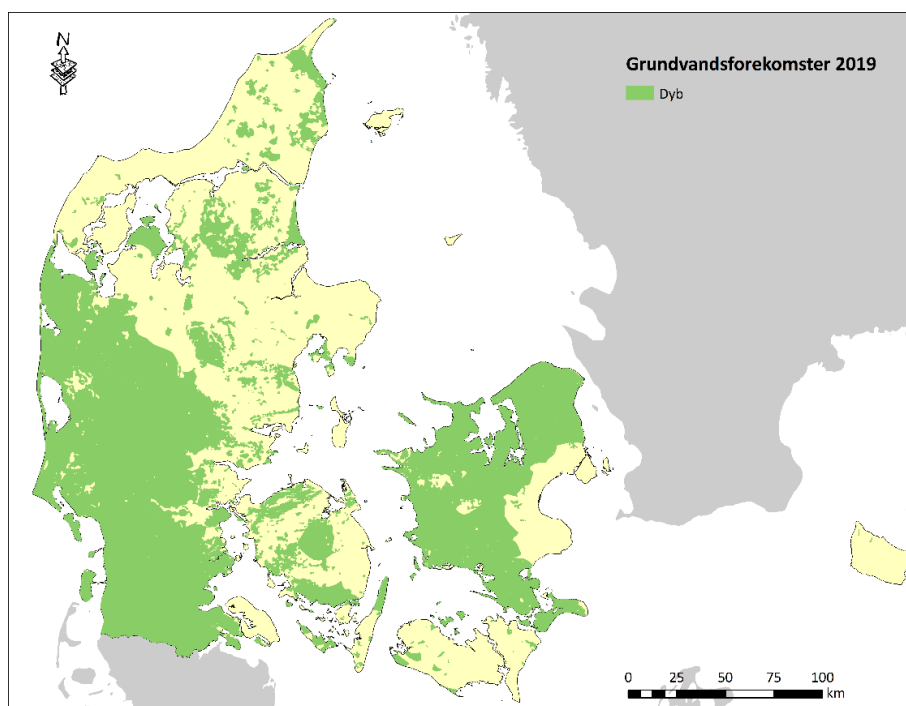
Figure 5.6. Distribution of deep groundwater bodies. 'Deep' designates maximum depth of 200-250 meters. From Trolborg (2020).
