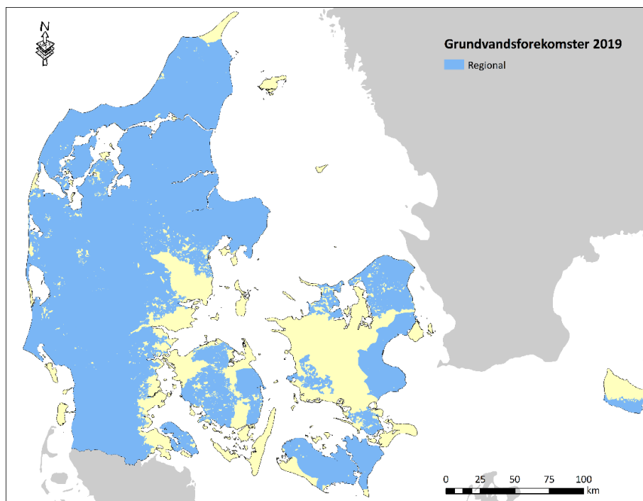
Figure 5.5. Distribution of regional groundwater bodies. From Trolborg (2020).
