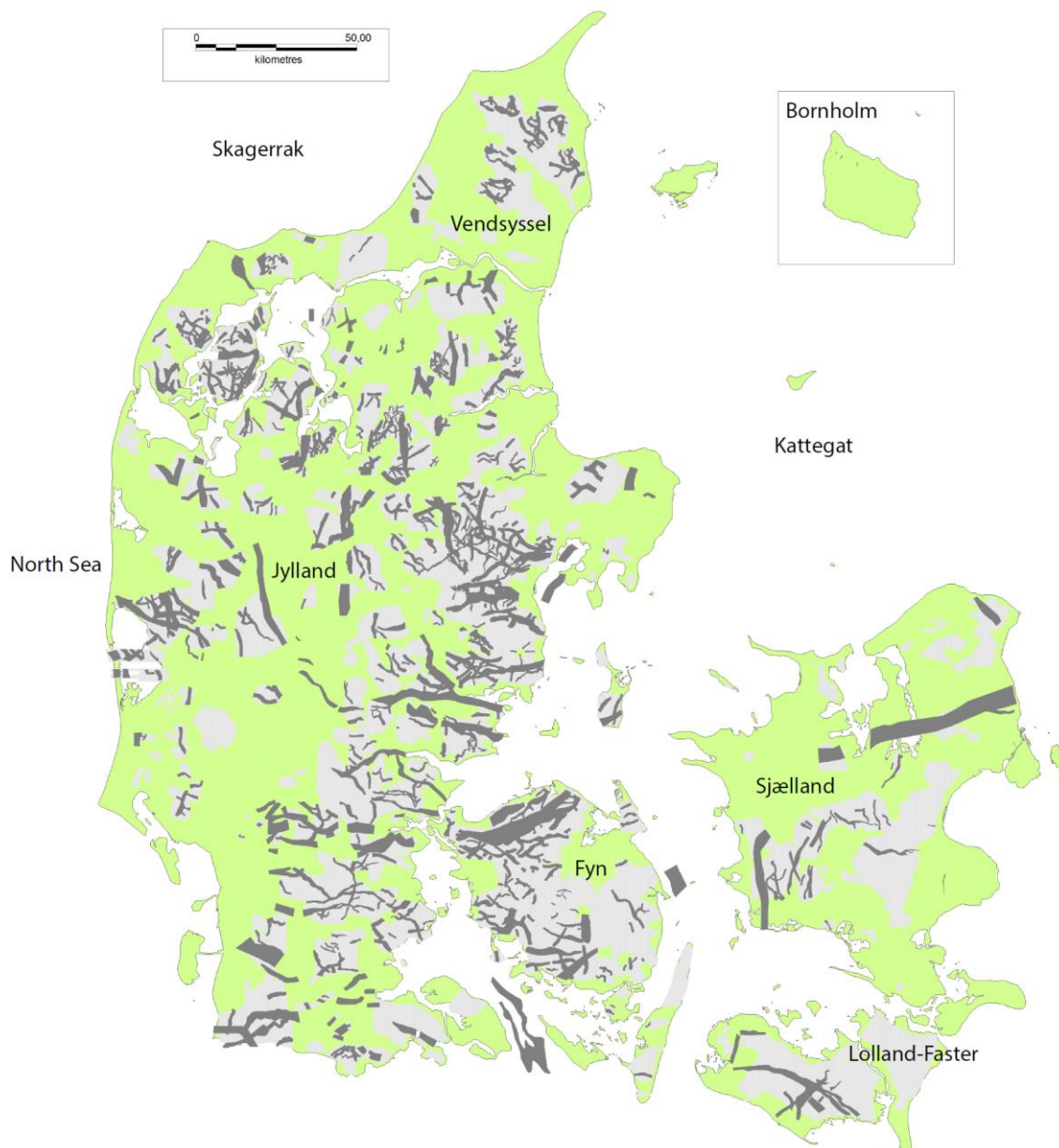
Figure 2.7. Mapped buried valleys in Denmark shown with dark-grey polygons. The light grey colour indicates areas mapped using the Transient ElectroMagnetic method (TEM). Modified from Sandersen & Jørgensen (2017).
