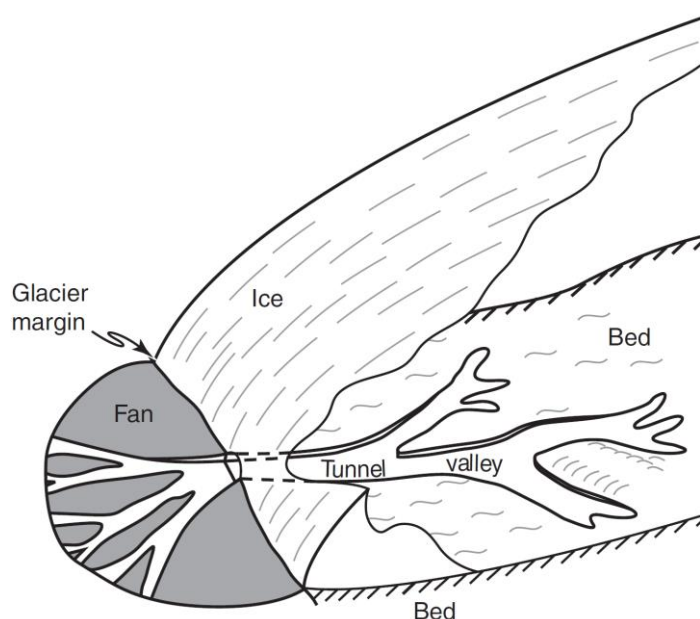
Figure 2.6. Sketch of a tunnel valley at the ice/bed interface close to the glacier margin. From Hooke & Jennings (2006).
