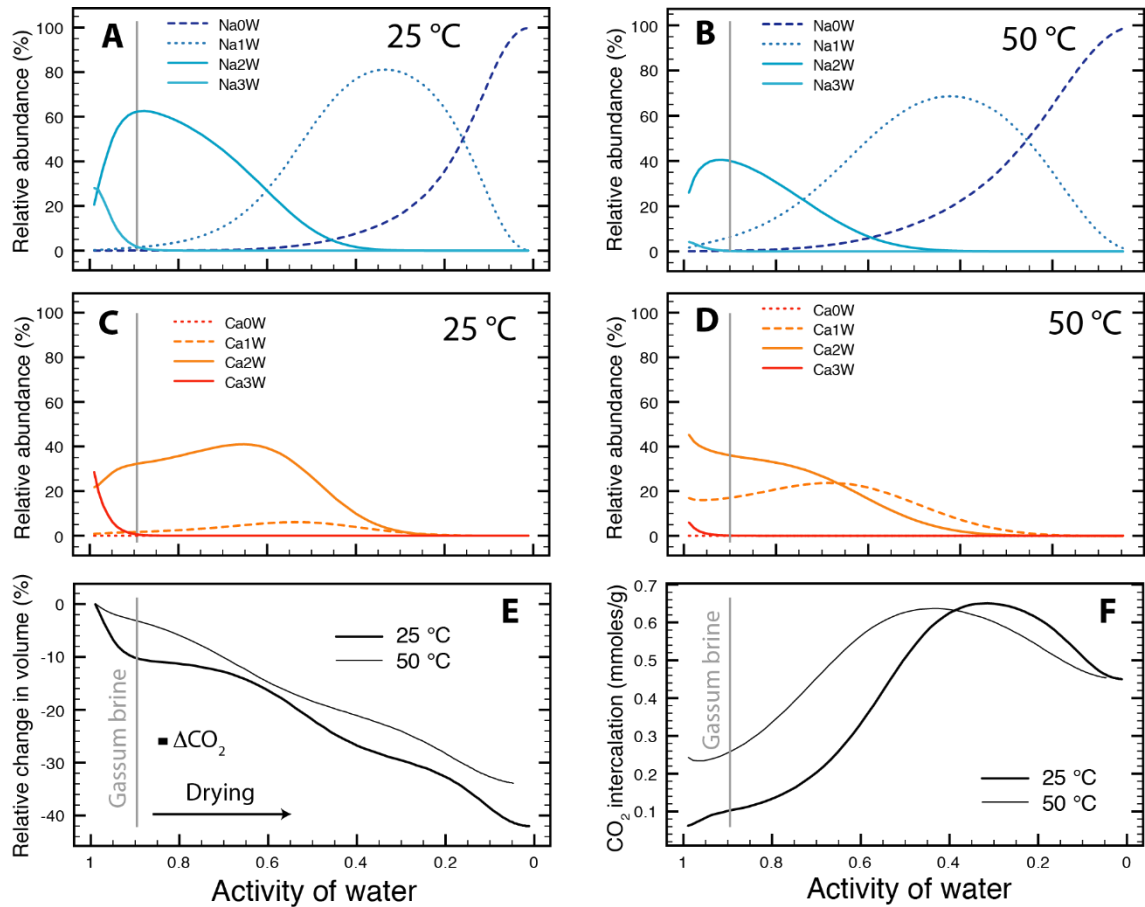
Figure 3.2. Calculated interlayer speciation as a function of the activity of water for Na (A and B) and Ca (C and D) at 25 and 50 °C. The relative change in volume and the CO 2 intercalation as a function of water activity are shown in E and F. The bar indicated by "DCO 2 " indicates the change in water activity occurring as a result of CO 2 dissolution at 50 °C and the water composition of the Fjerritslev brine.
