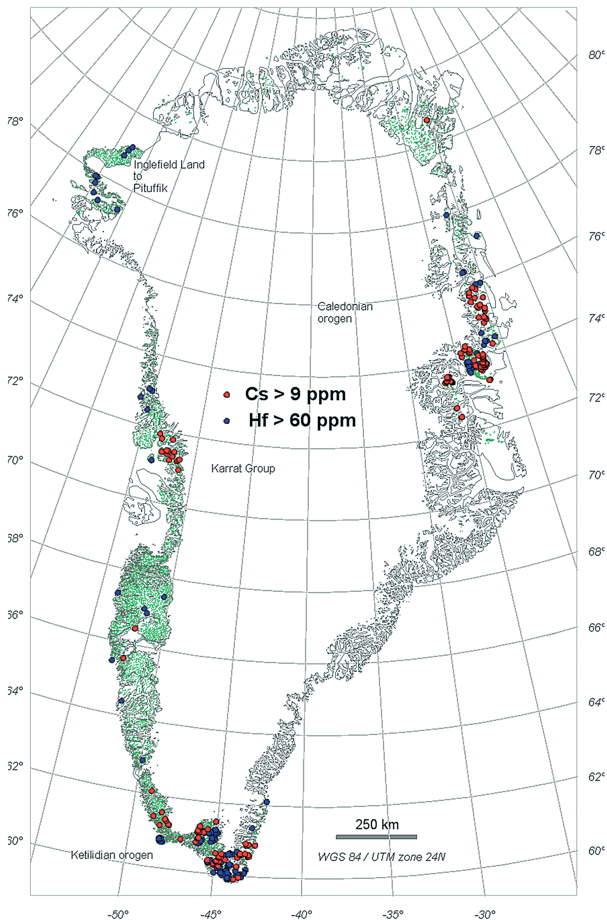
Locations of stream sediment samples with high concentrations of Cs and Hf in the < 0.1 mm fraction. Green dots mark location of samples analysed by neutron activation.
