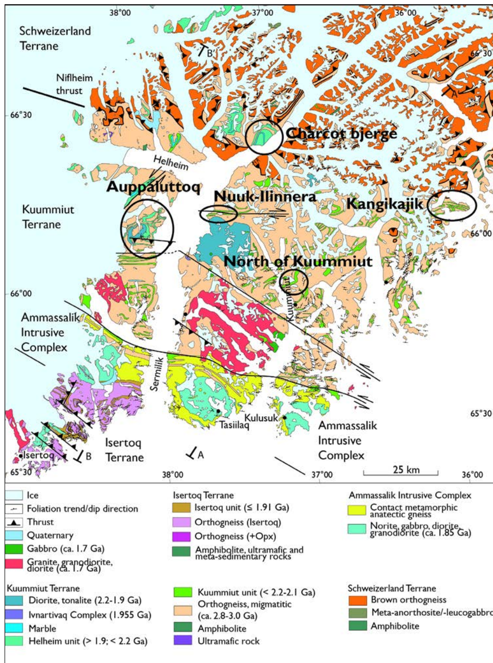
Figure 24. Geological map of the Ammassalik mobile belt, with the Aupaluttoq and the Kangikajik occurrence. (Source: Rosing-Schow et al. 2017).
