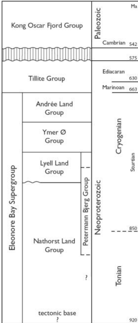
Figure 44. Lithostratigraphic subdivision of the Neoproterozoic Eleonore Bay Basin. From Sønderholm et al. 2008.
