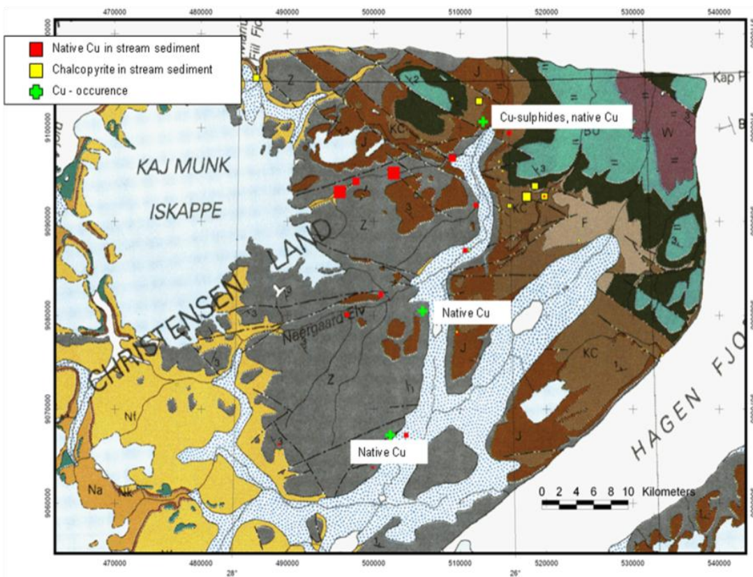
Figure 84. Copper mineralizations in the Hagen Fjord Group For full legend, see Bengaard & Henriksen (1986). From workshop presentation by Tukiainen & Lind.
