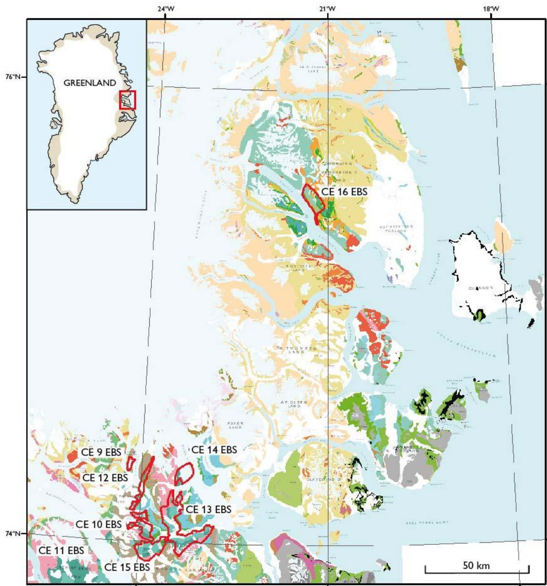
Figure 42B. Distribution of the Neoproterozoic tract CE 9-15 EBS and Tract CE 16 EBS. The tracts contain the Neoproterozoic Elenore Bay Supergroup (EBS) assessed for undiscovered Reduced Facies Copper type deposits at the boundary zone between the Lyell Land Group and Ymer Ø Group.
