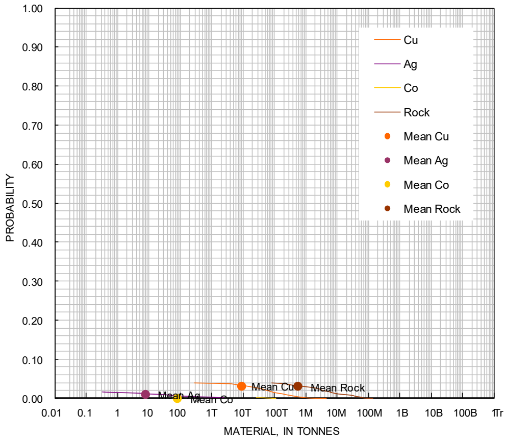
Figure 67. Cumulative frequency plot showing the results of a Monte Carlo computer simulation of undiscovered resources in the tracts NW 3-4 Narssârssuk Group Redbed type. T=thousands, M=millions, B=Billions, Tr=Trillions.
