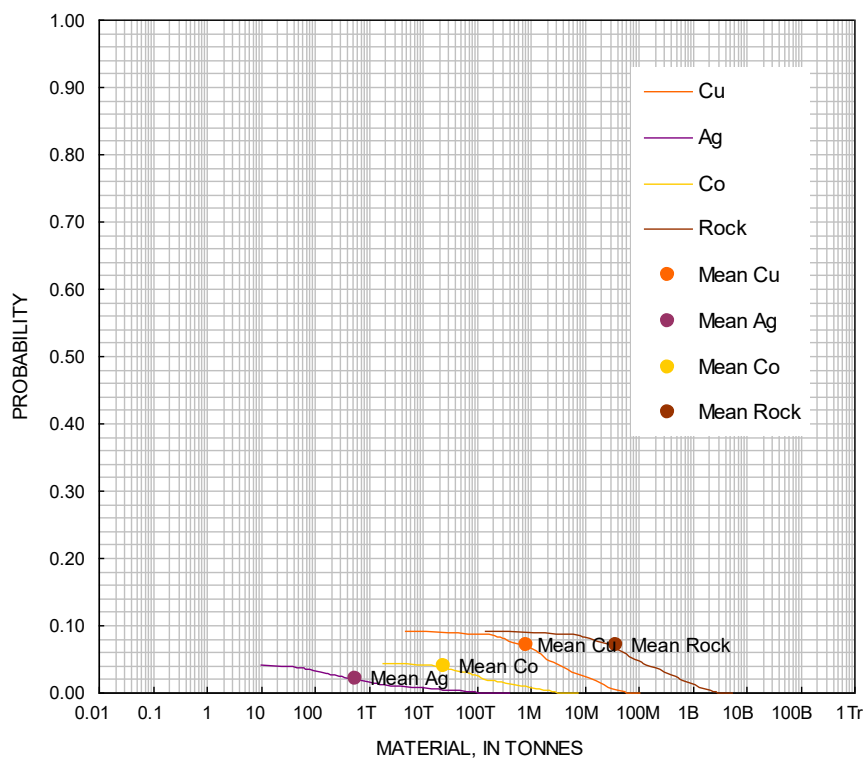
Figure 37. Cumulative frequency plot showing the results of a Monte Carlo computer simulation of undiscovered resources in the Upper Triassic tract CE1A Pingel Dal Bed, Reduced Facies Copper type deposits. T=thousands, M=millions, B=billions, Tr=trillions.
