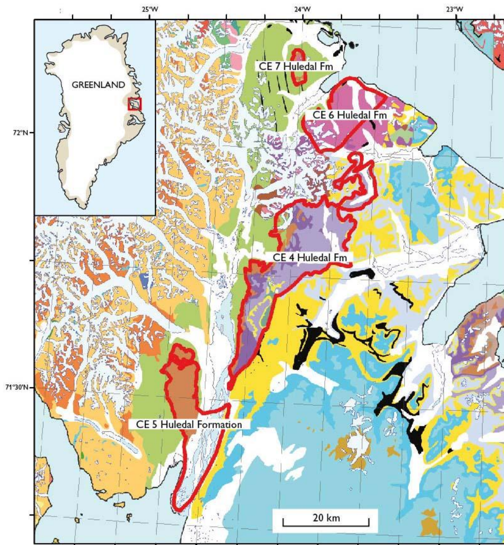
Figure 10. Tracts CE 4-7 Huledal Formation in the western part of the Jameson Land sedimentary basin; the Huledal Formation is shown in brown. See Appendix B for a geological legend.
