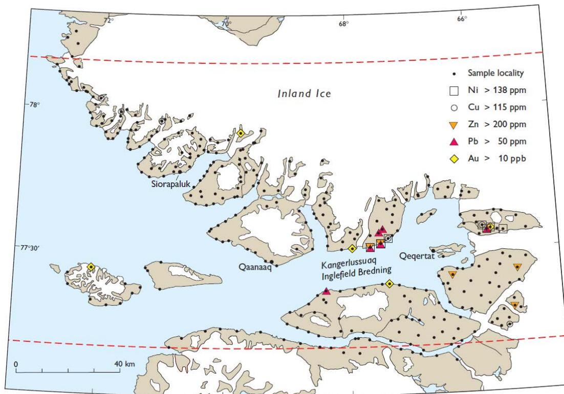
Figure 56. Map of the Qaanaaq region showing anomalous concentrations of copper and other selected elements based on stream sediment samples. From Thomassen et al. 2002.
