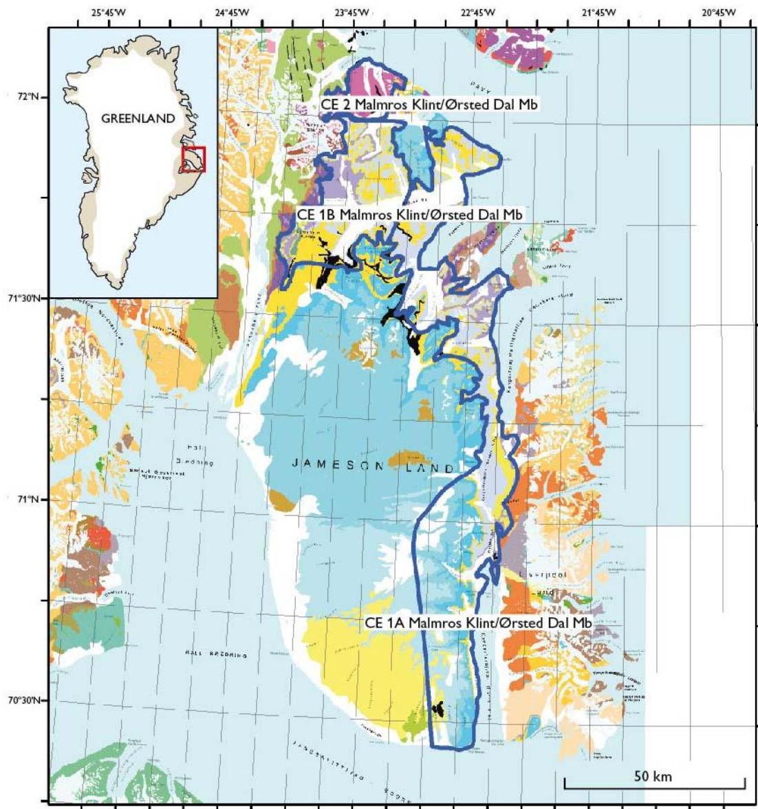
Figure 29. The Upper Triassic tracts CE 1A, CE 1B, and CE 2 Malmros Klint/ Ørsted Dal Member, in the Jameson Land basin. CE 1 A and CE 1 B Malmros Klint/ Ørsted Dal Member are assessed for undiscovered Redbed Copper type deposit.
