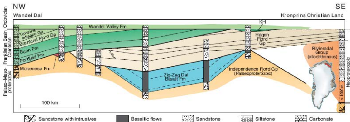
Figure 82. Schematic cross-section of the Proterozoic–Ordovician succession in eastern North Greenland between 82^{\circ}\text{N} and Kronprins Christian Land \sim 80^{\circ}\text{N} . From Henriksen et al. 2009.
