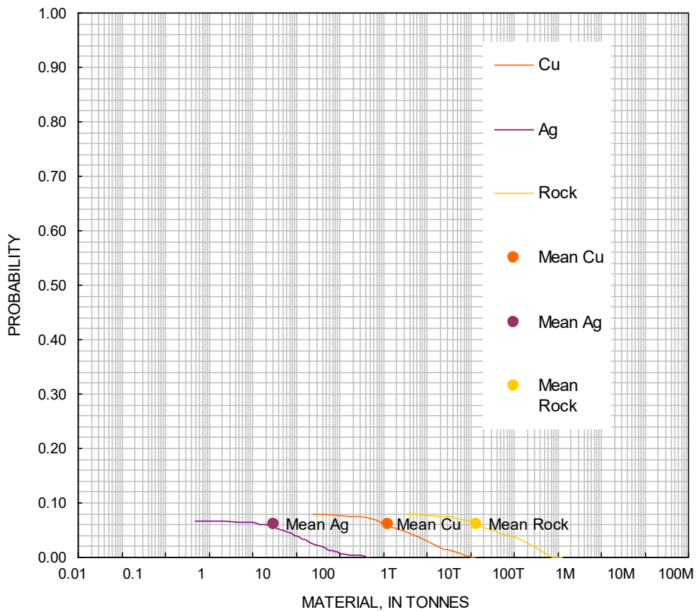
Figure 22. Cumulative frequency plot showing the results of a Monte Carlo computer simulation of undiscovered resources in the Permian tract CE13–14 Huledal Formation. T=thousands, M=millions.
