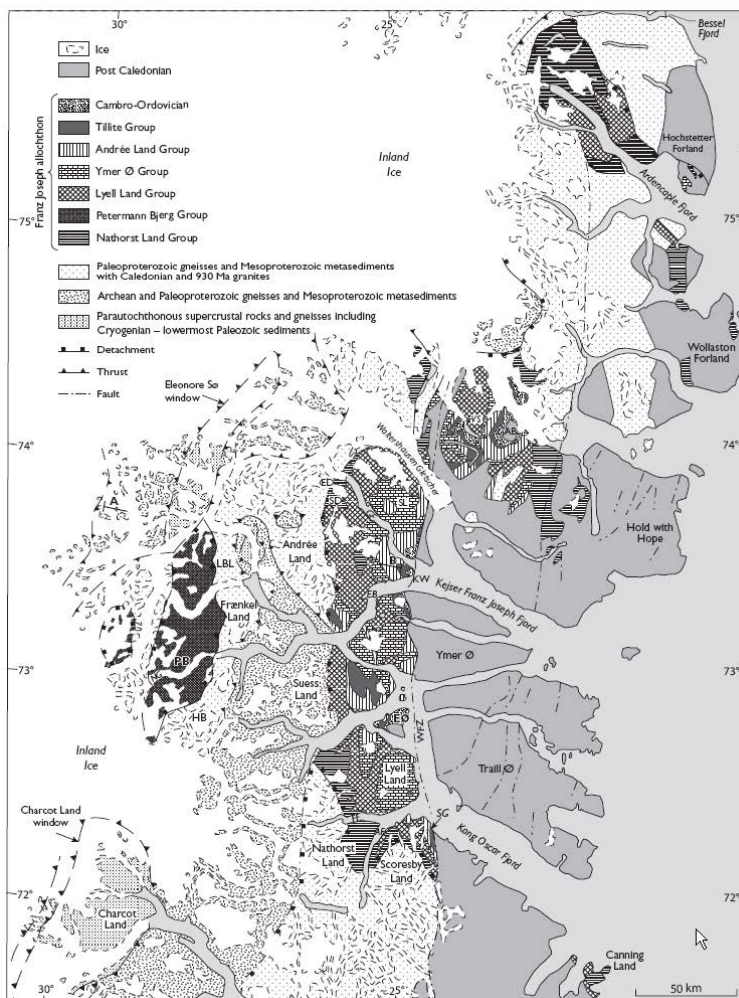
Figure 43. Simplified geological map showing the distribution of the sediments of the Neoproterozoic Eleonore Bay Basin. From Sønderholm et al. 2008.
