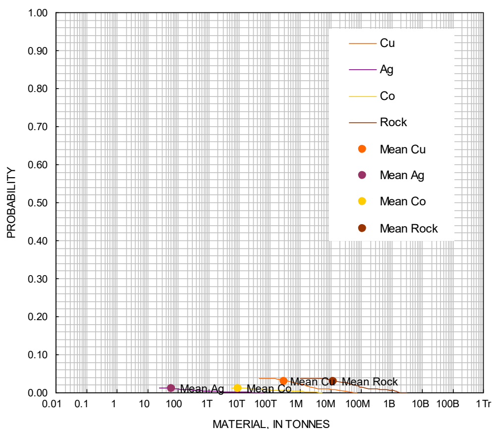
Figure 41. Cumulative frequency plot showing the results of a Monte Carlo computer simulation of undiscovered resources in the Upper Triassic tract CE 1B Pingel Dal Bed, Reduced Facies Copper type deposits. T=thousands, M=millions, B=billions, Tr=trillions.
