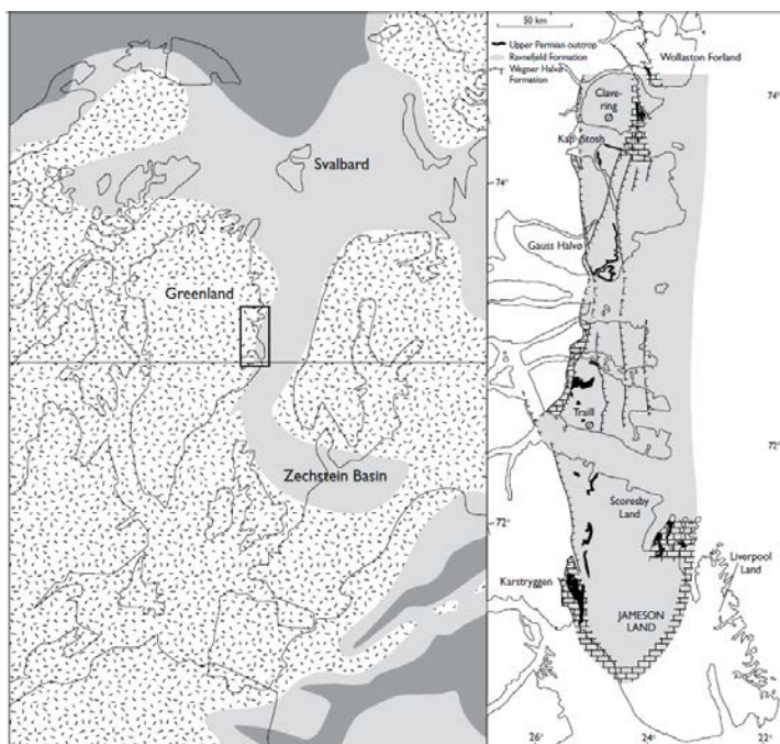
Figure 5. Reconstruction of the Upper Permian North Atlantic showing the position of East Greenland. The East Greenland map shows the outline of the Upper Permian depositional basin with distribution of exposed Upper Permian stratum shown in black. Figure from Sørensen et al. 2008.
