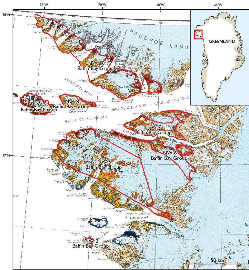
Figure 55. Tracts NW 1–2 and NW 5–10 Baffin Bay Group, assessed for undiscovered Redbed Copper type deposit.
