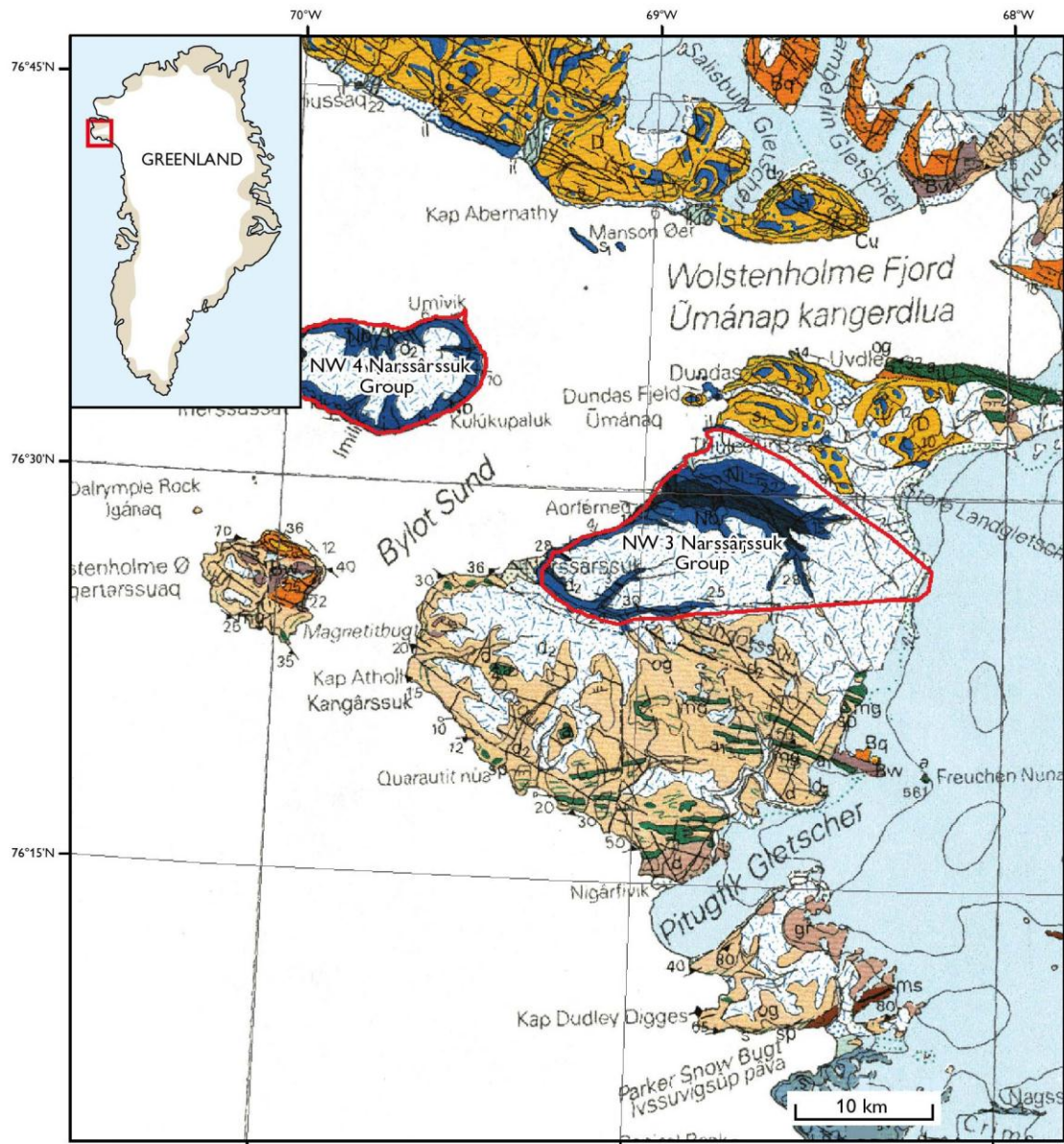
Figure 66. Tracts NW 3–4 Narssârssuk Group in North West Greenland, assessed for undiscovered Redbed Copper type deposit plotted on top of the 1:500 000 geological map for the area (Dawes 1991). In dark blue (Ni and Nb) the Narssârssuk Group. Refer to this map for a full legend.
