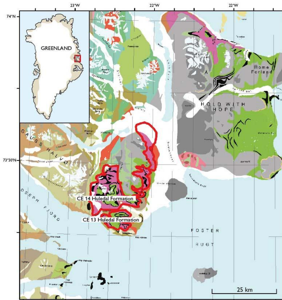
Figure 21. Outline of the Permian tracts CE 13 and CE 14 Huledal Formation at Gauss Halvø. Location of the Ladderbjerg Copper deposit is indicated by red dot. The Huledal Formation is shown in brown; Triassic units are shown in pink. See Appendix B for the geological legend.
