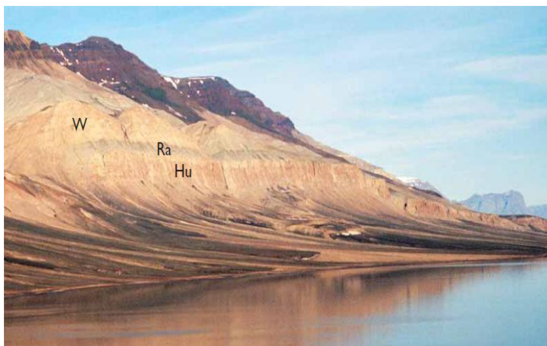
Figure 24. The Permian-Triassic boundary at Kap Stosch. The dark Upper Permian Ravnefjeld Formation (Ra) is directly overlain by the Wordie Creek Formation (W) which is unconformably overlain by Tertiary basalts forming the top of the approximately 1300 m high mountains; (Hu) is Huledal Formation. Photo from Stemmerik et al. (2001).
