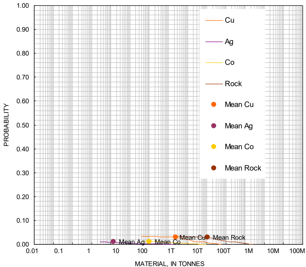
Figure 27. Cumulative frequency plot showing the results of a Monte Carlo computer simulation of undiscovered resources in the tracts CE 2 and CE 4-15 Ravnefjeld Formation. T=thousands, M=millions.
