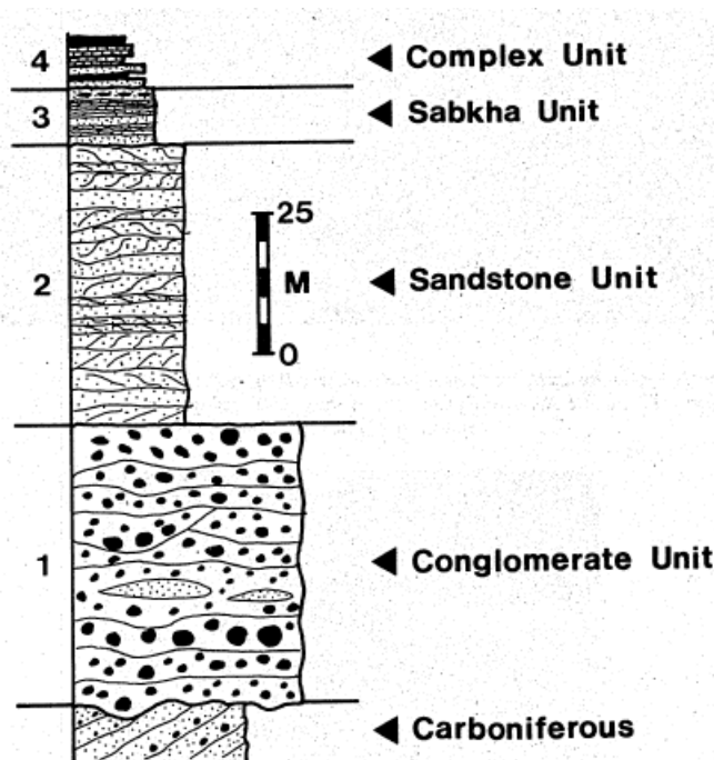
Figure 10. Generalised Upper Permian sequence of the Rubjerg Knude area, central Trail Ø – tract CE 9 Huledal Formation. From Harpøth (1982).
