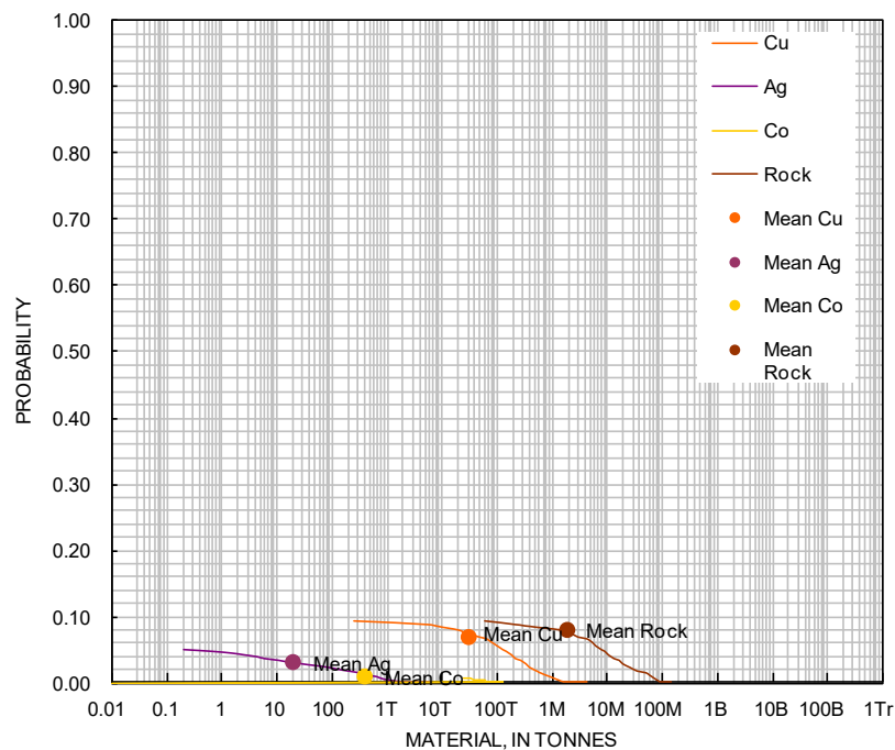
Figure 72. Cumulative frequency plot showing the results of a Monte Carlo computer simulation of undiscovered resources in the tracts NW 11–13 Smith Sound Group Redbed type. T=thousands, M=millions, B=Billions, Tr=Trillions.
