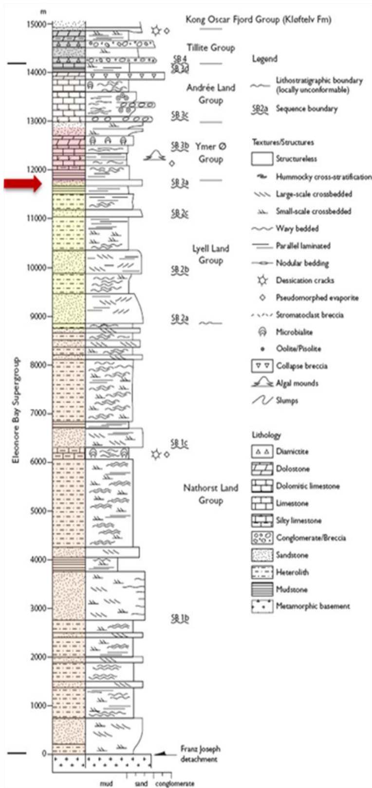
Figure 45. Generalized section of the Eleonore Bay Supergroup. The red arrow indicates the most widespread and persistent copper mineralization - the „mineralised horizon number 7“ (Table 38) included in the assessment. From Sænderholm et al. (2008).
