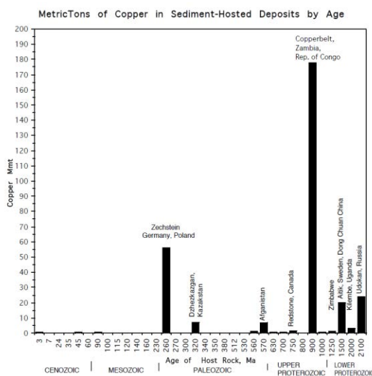
Figure 1. Distribution of copper (million metric tons) in sedimentary-hosted copper deposits of different ages (from Cox et al. 2007).
