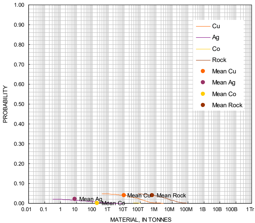
Figure 34. Cumulative frequency plot showing the results of a Monte Carlo computer simulation of undiscovered resources in the Upper Triassic tract CE 1B Malmros Klint/ Ørsted Dal Member, Redbed Copper type. T=thousands, M=millions, B=billions, Tr=trillions.
