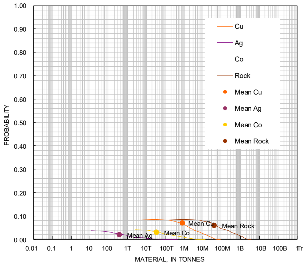
Figure 52. Cumulative frequency plot showing the results of a Monte Carlo computer simulation of undiscovered resources in the tracts CE 7-8 EBS, Reduced Facies Copper type deposits. T=thousands, M=millions, B=billions, Tr=trillions.
