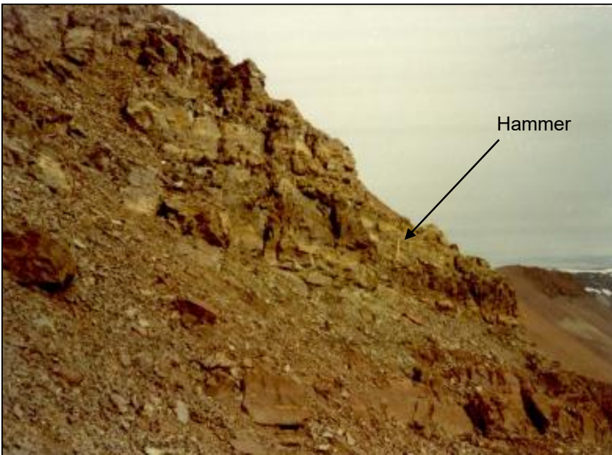
Figure 40. Pingel Dal Bed at Malmros Klint. Cu-bearing, yellowish beds (hammer 45 cm) underlain by red, unmineralised mudstones. Photo from Thomassen & Svensson (1979).
