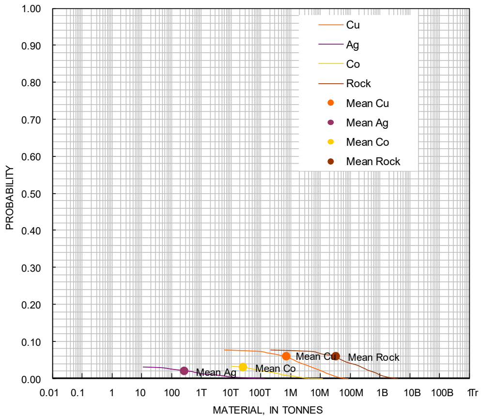
Figure 48. Cumulative frequency plot showing the results of a Monte Carlo computer simulation of undiscovered resources in the tracts CE 1-6 EBS and CE 9-16 EBS Eleonore Bay Super-group, Reduced Facies Copper type deposits, Greenland. T=thousands, M=millions, B=billions, Tr=trillions.
