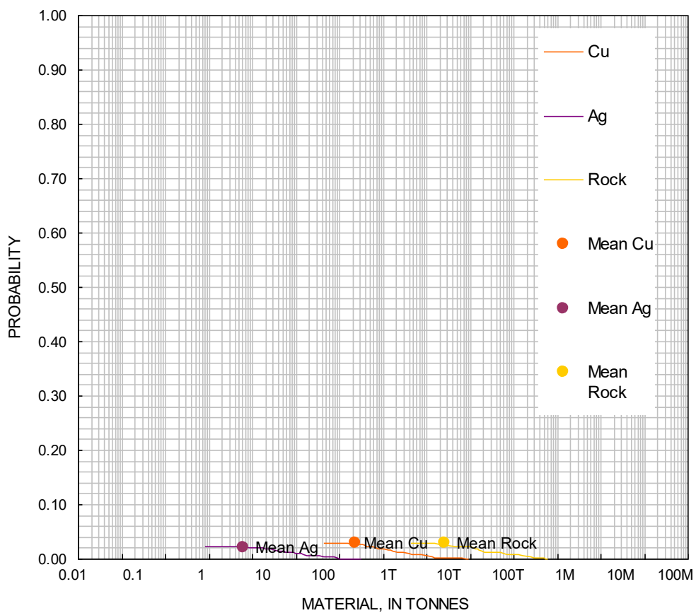
Figure 25. Cumulative frequency plot showing the results of a Monte Carlo computer simulation of undiscovered resources in the tract CE 15 Huledal Formation. T=thousands, M=millions.
