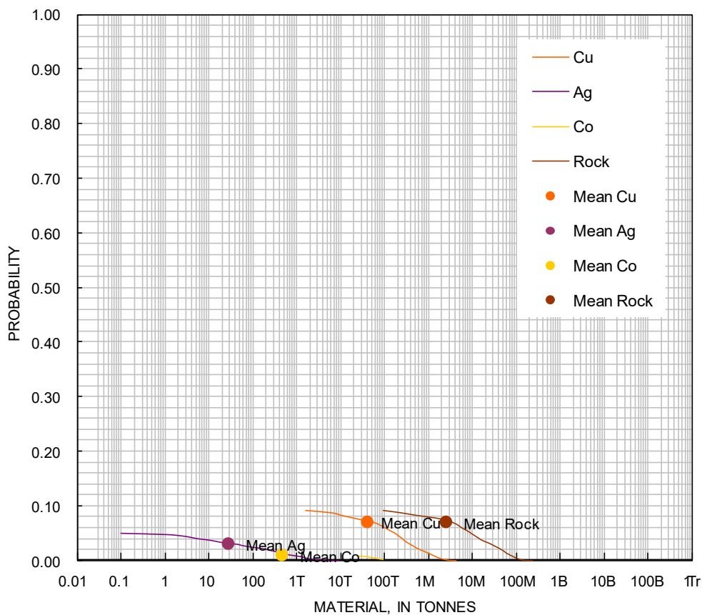
Figure 60. Cumulative frequency plot showing the results of a Monte Carlo computer simulation of undiscovered resources in the tracts NW 1–2 and NW 5–10 Baffin Bay Group Redbed type. T=thousands, M=millions, B=Billions, Tr=Trillions.
