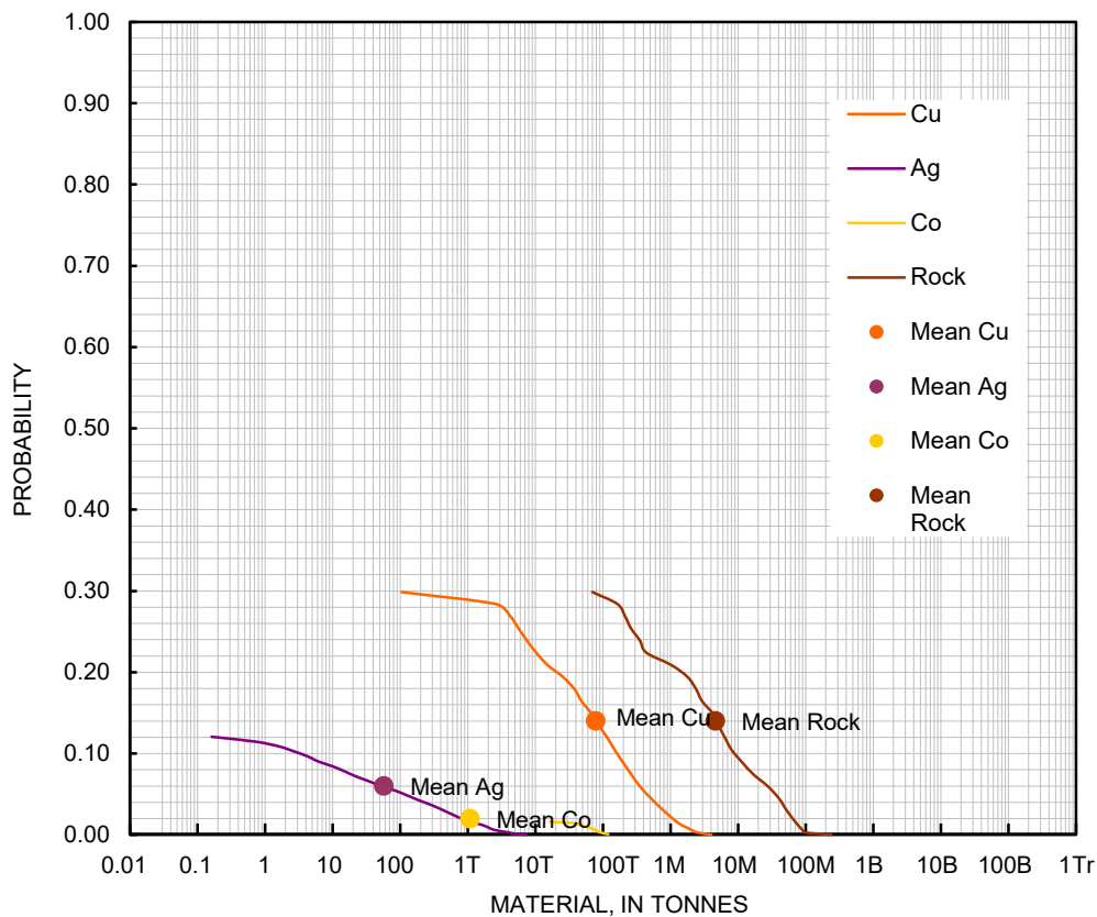
Figure 62. Cumulative frequency plot showing the results of a Monte Carlo computer simulation of undiscovered resources in the tracts NW 5–10 Nares Strait Group Redbed type. T=thousands, M=millions, B=Billions, Tr=Trillions.
