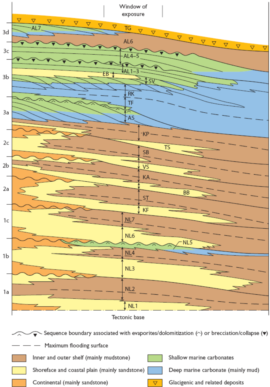
Figure 46. Tentative sequence stratigraphic cross section for the four stage basin evolution of the Eleonore Bay Basin. From Sønderholm et al. (2008).
