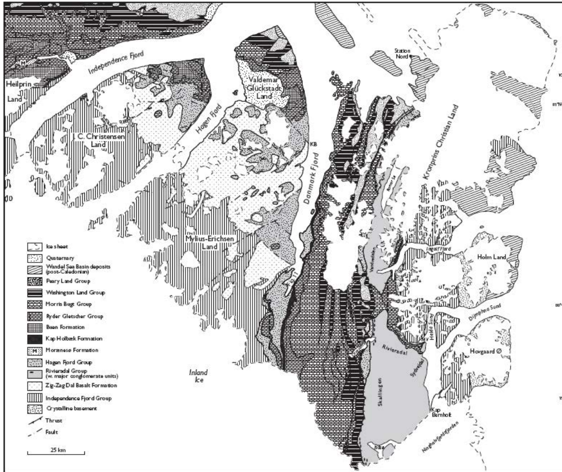
Figure 81. Simplified map showing the distribution of Hagen Fjord Group, the underlying Zig-Zag Dal Basalt Formation and the Independence Fjord Group. From workshop presentation given at the workshop by M. Sænderholm.
