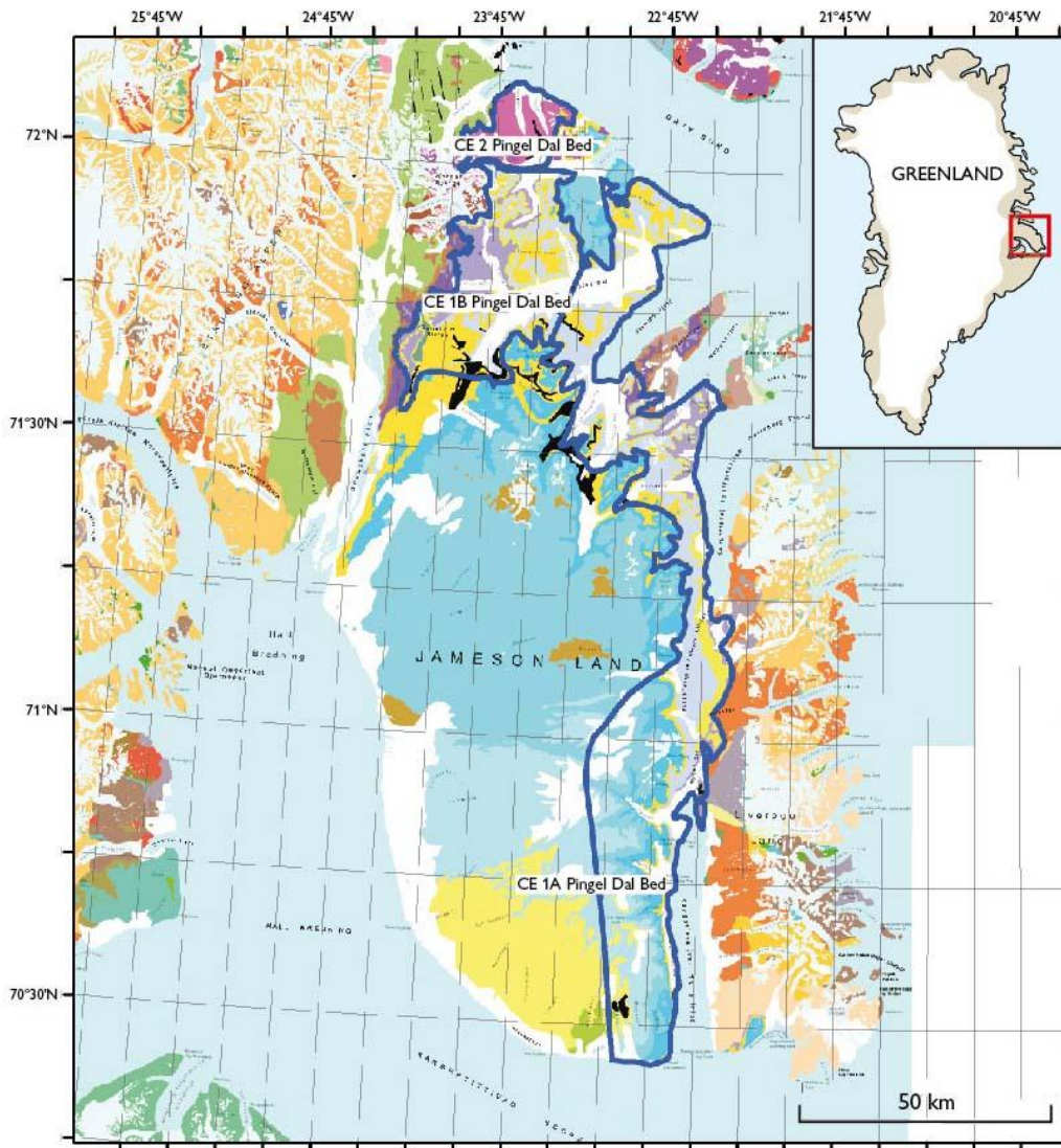
Figure 36. The Upper Triassic tracts CE 1A-, CE 1B- and CE2 Pingel Dal Bed in the Jameson Land basin. CE 1A and CE 1B Upper Triassic are assessed for undiscovered Reduced Facies Copper type deposits within the Pingel Dal Bed.
