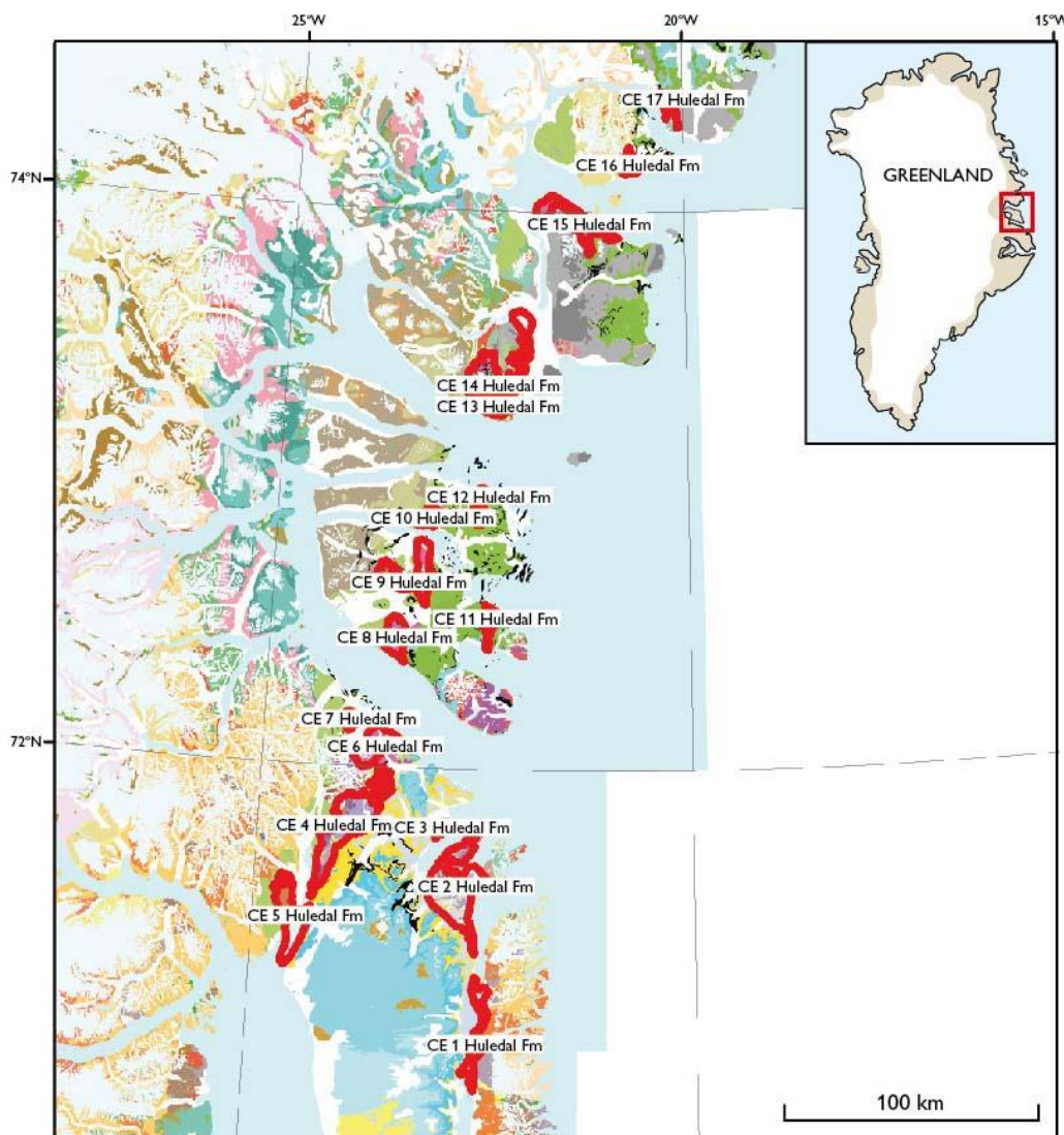
Figure 2. Tracts for Upper Permian hosted Revett Copper type (Tracts CE1-17 Huledal Formation). Tracts CE 1, CE 3, CE16 and CE 17 Huledal Formation were excluded.
