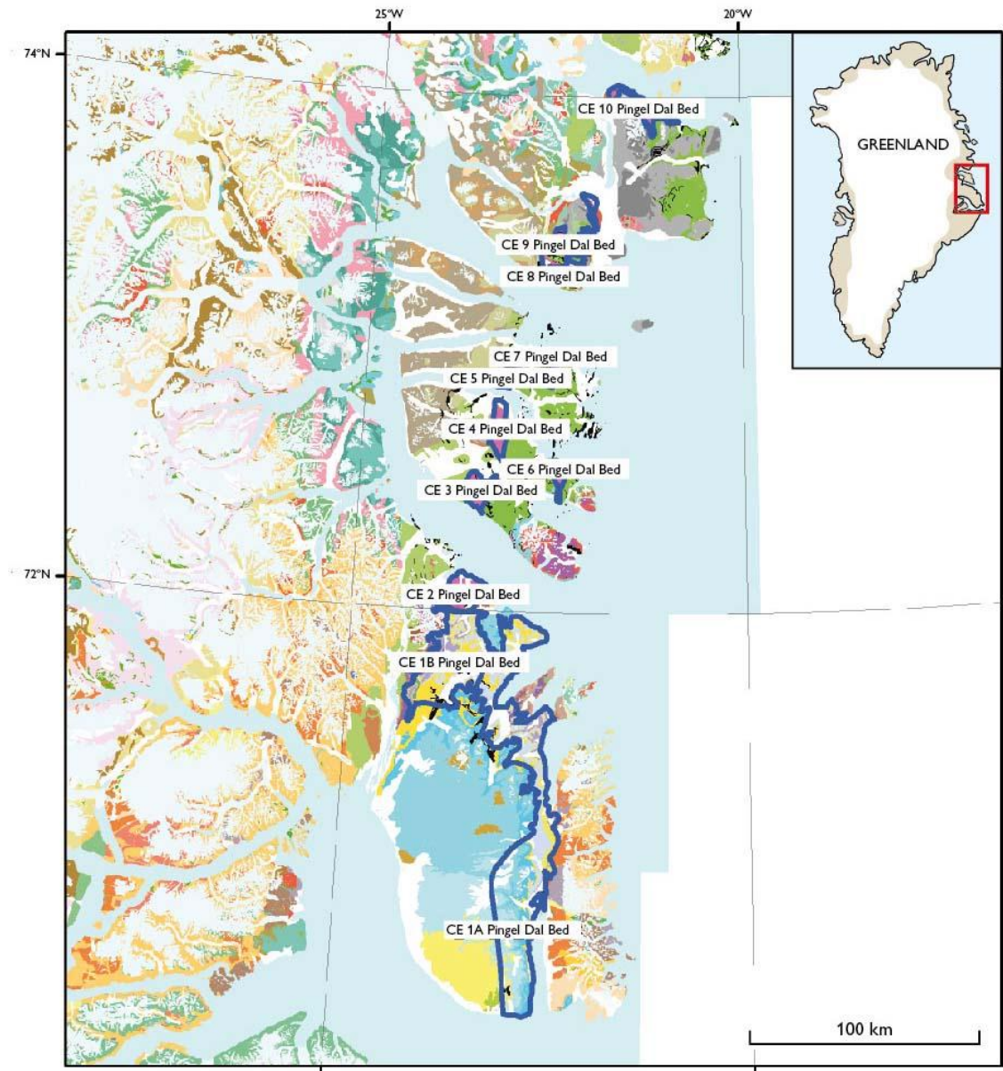
Figure 35. Tracts for Upper Triassic Pingel Dal Bed hosting Reduced Facies Copper deposit type. Tract CE 2 to CE 10 Upper Triassic are excluded from the assessment.
