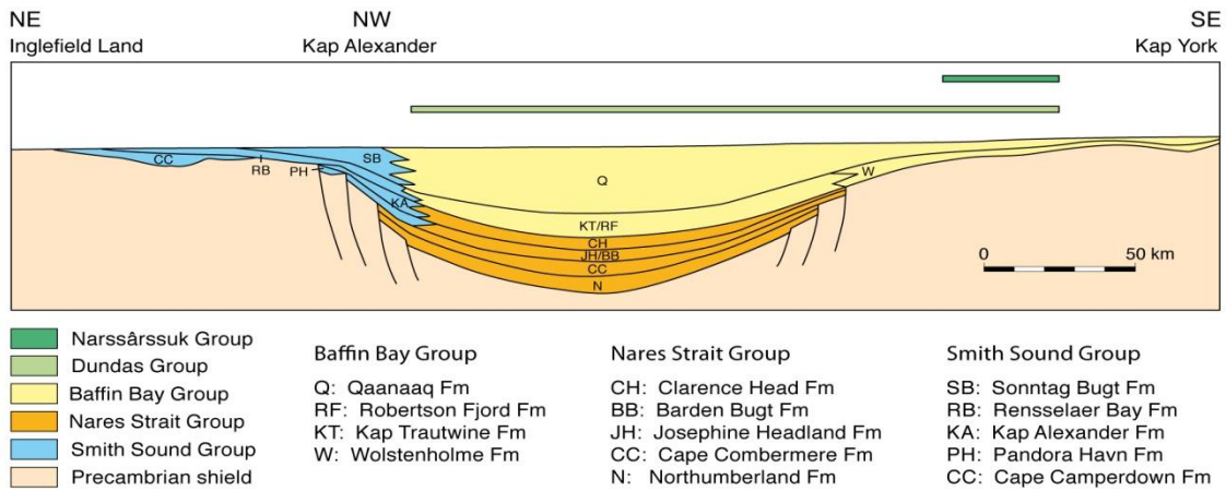
Figure 54. Cross-section of the lower Thule Supergroup. Figure from the workshop presentation by Peter Dawes.
