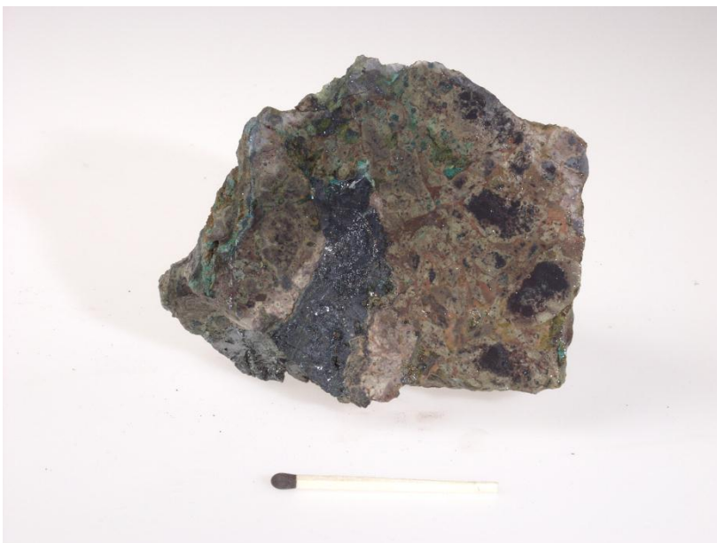
Figure 79. Hematite-chalcocite-bearing volcanic float with 1.7% Cu, 21.9% Fe. Lose scree-block from Parish Gletscher beneath exposed Cape Combermere Formation. Match is 5 cm. Photos from workshop presentation by B. Thomassen.
