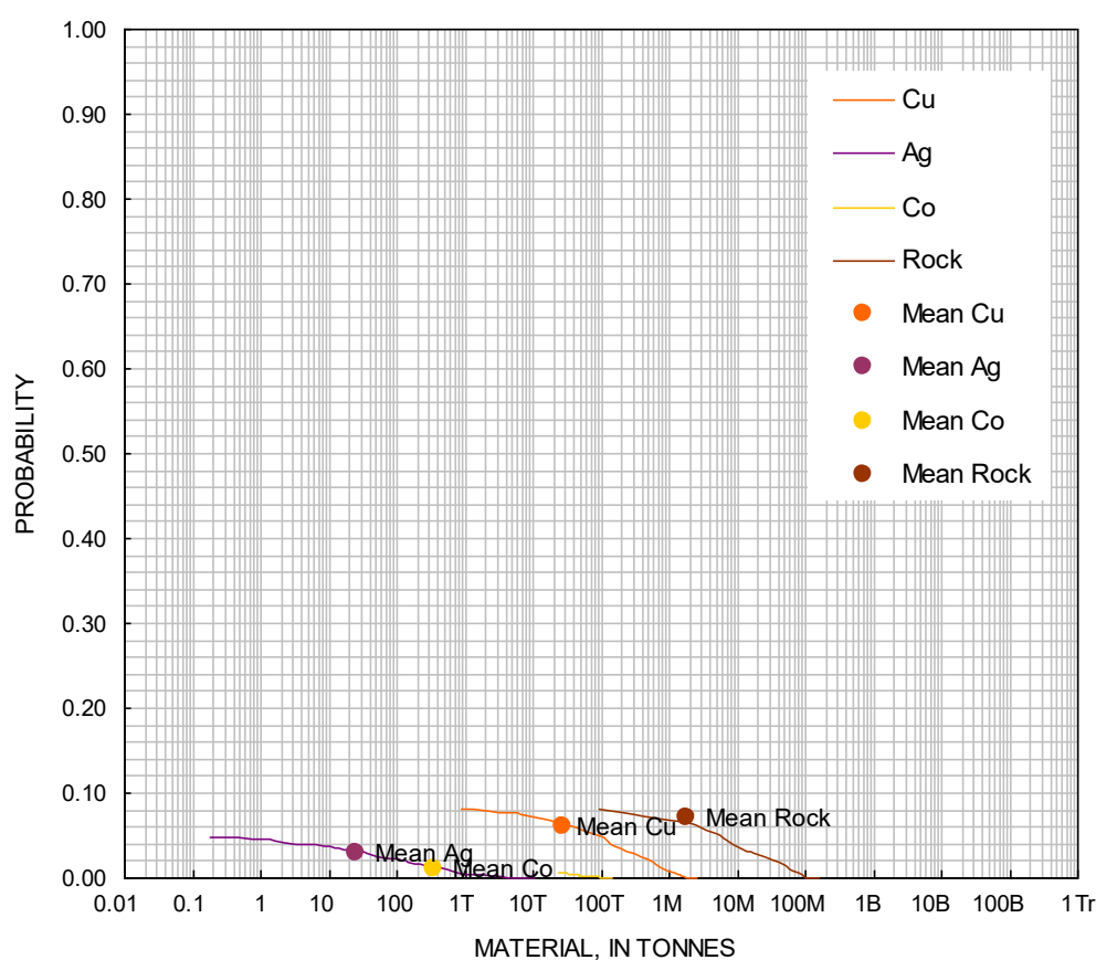
Figure 31. Cumulative frequency plot showing the results of a Monte Carlo computer simulation of undiscovered resources in the Upper Triassic tract CE 1A Malmros Klint/ Ørsted Dal Member, Redbed type. T=thousands, M=millions, B=Billions, Tr=Trillions.
