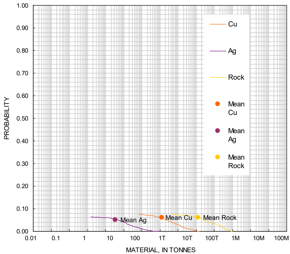
Figure 11. Cumulative frequency plot showing the results of a Monte Carlo computer simulation of undiscovered resources in the tract CE4–7 Huledal Formation. T=thousands, M=millions.
