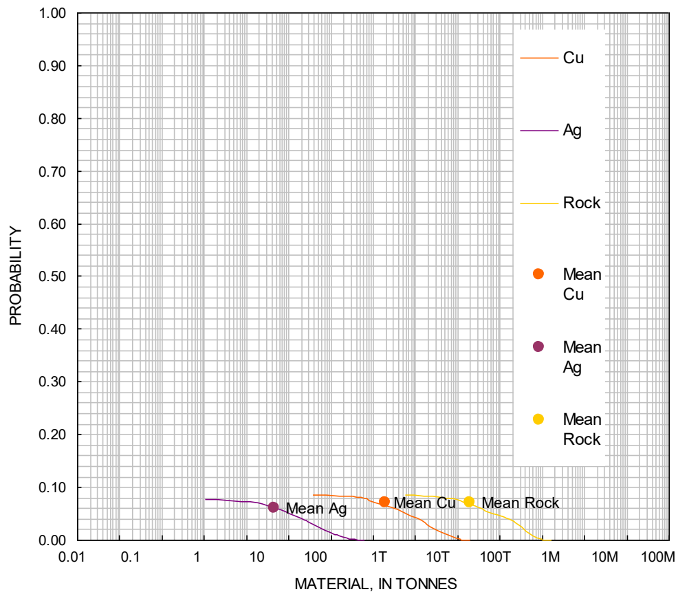
Figure 20. Cumulative frequency plot showing the results of a Monte Carlo computer simulation of undiscovered resources in the Permian tract CE 8–12 Huledal Formation. T=thousands, M=millions.
