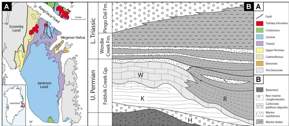
Figure 4. A. Simplified geological map of central East Greenland. B. Simplified geological cross section from Upper Permian to Lower Triassic sedimentary succession in Jameson Land Basin. H = Huledal Formation, K = Karstryggen Formation, W = Wegner Halvø Formation, R = Ravnefjeld Formation, S = Schuchert Dal Formation. Figure from workshop presentation by J.K. Nielsen and M. Pedersen.
