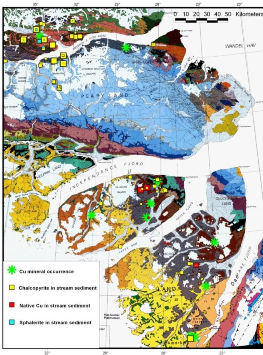
Figure 83. Distribution of known copper occurrences and chalcopyrite, native Cu, and sphalerite from stream sediment samples in the region between Danmark Fjord and Frederik E. Hyde Fjord. Hagen Fjord Group is shown in brown and beige, while the underlying Zig-Zag Dal Basalt Formation in grey. For full legend refer to Bengaard and Henriksen (1986). From presentation given at the workshop by Tukiainen & Lind.
