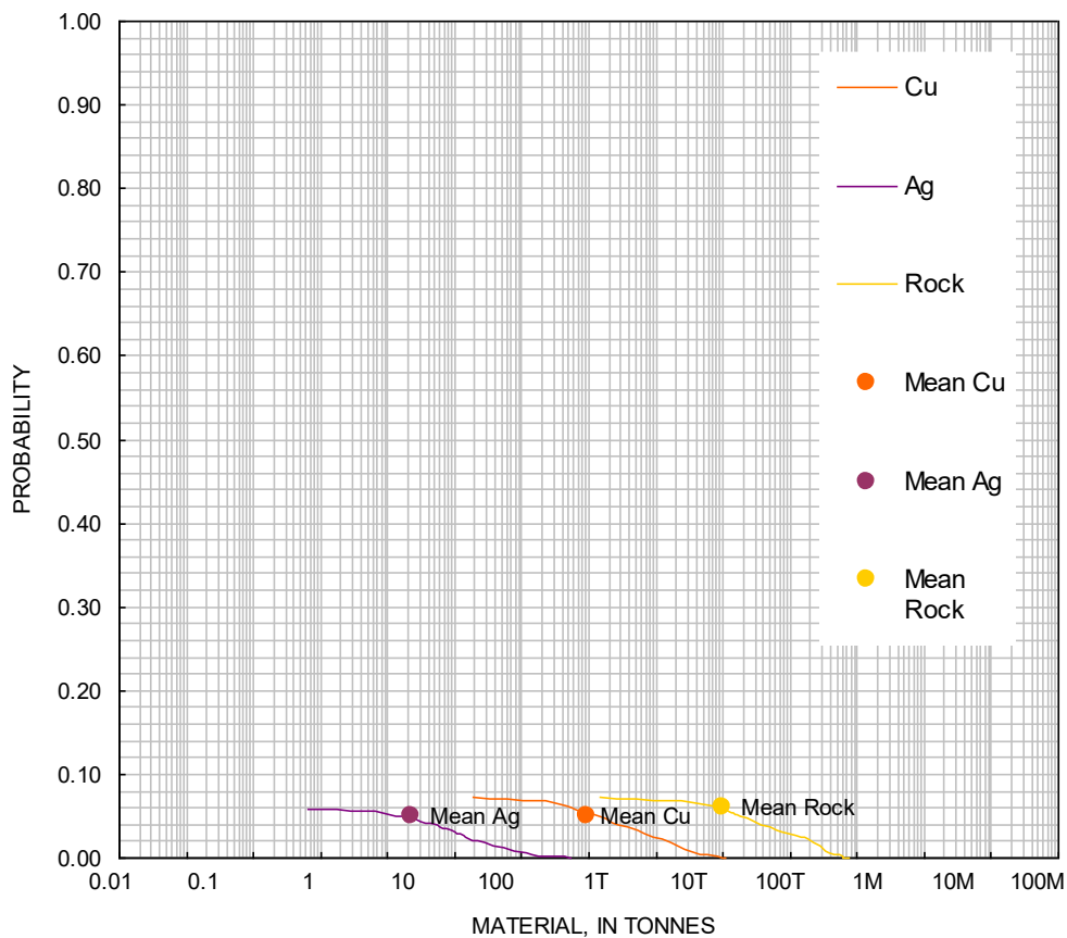
Figure 9. Cumulative frequency plot showing the results of a Monte Carlo computer simulation of undiscovered resources in the tract CE 2 Huledal Formation. T=thousands, M=millions.
