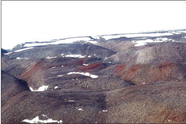
Figure 85. Jyske Ås Formation sandstones with rusty alteration along lineaments extending westwards from one of the copper occurrences at J.C. Christensen Land. From workshop presentation by Tukiainen & Lind.
