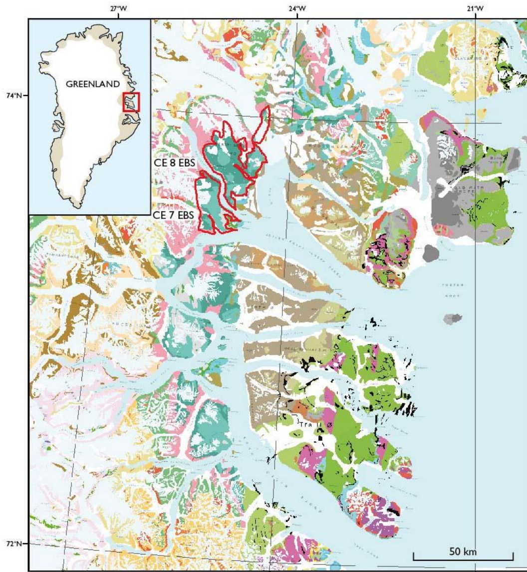
Figure 51. The tracts Neoproterozoic CE 7-8 EBS of the Eleonore Bay Supergroup (EBS) assesses for undiscovered Reduced Facies Copper type deposits at the boundary zone between the Lyell Land Group and Ymer Ø Group.
