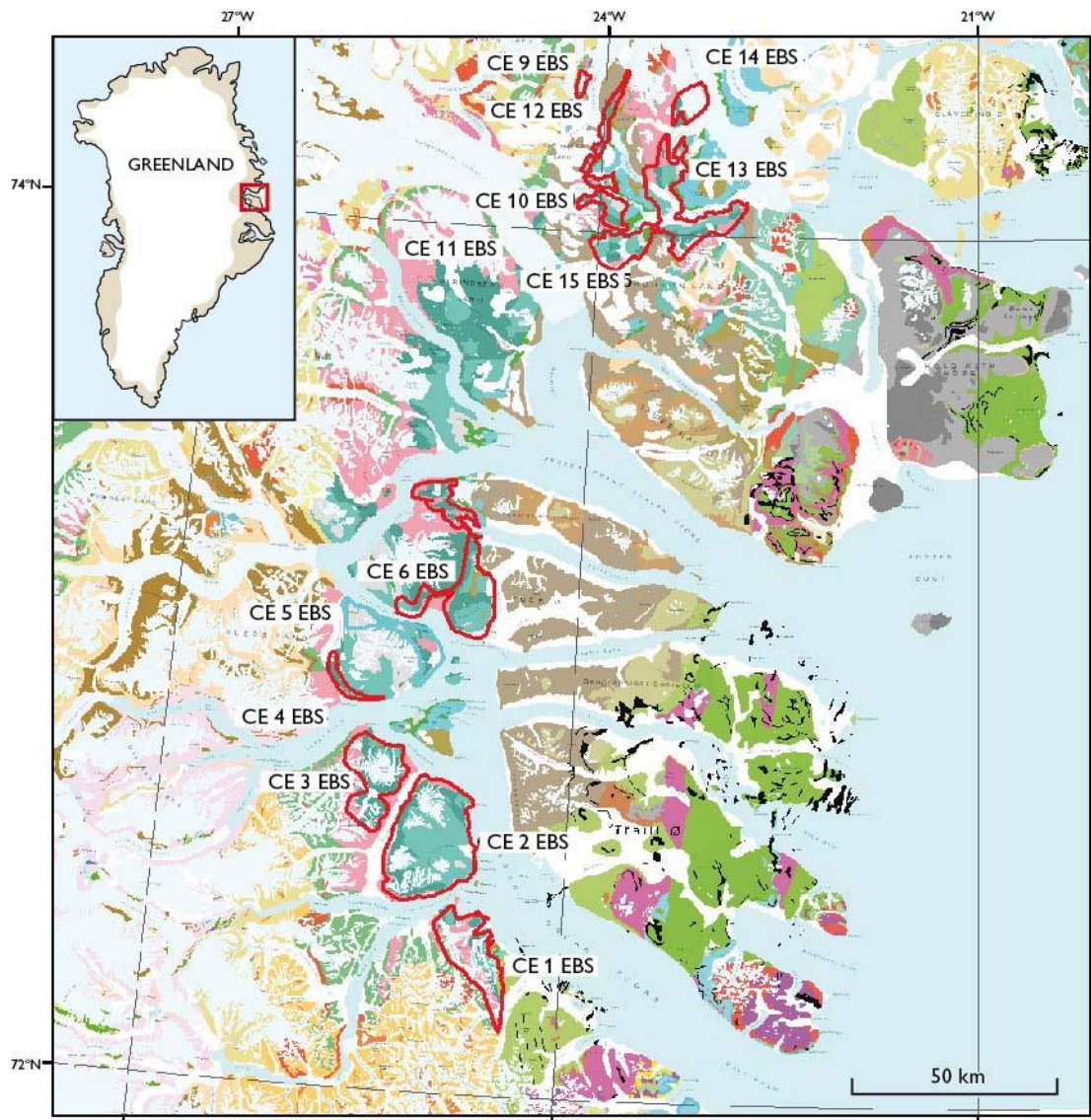
Figure 42A. Distribution of the Neoproterozoic tracts CE 1-6 EBS and CE 9-15 EBS, The tracts contain the Neoproterozoic Eleonore Bay Supergroup (EBS) assessed for undiscovered Reduced Facies Copper type deposits at the boundary zone between the Lyell Land Group and Ymer Ø Group.
