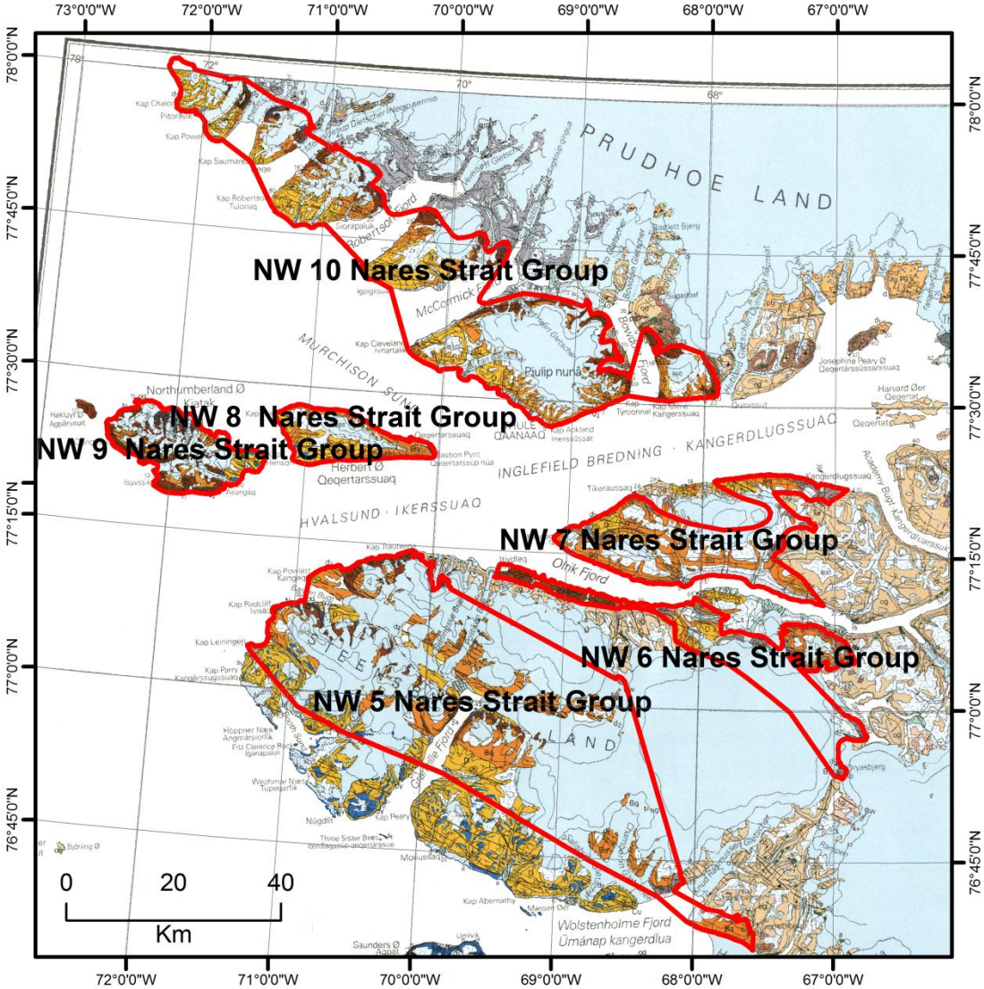
Figure 61. Tracts NW 5–10 Nares Strait Group in North West Greenland, assessed for undiscovered Redbed Copper type deposit plotted on top of the 1:500 000 geological map for the area (Dawes 1991). In dark grey (N) the Nares Strait Group. Refer to this map for a full legend.
