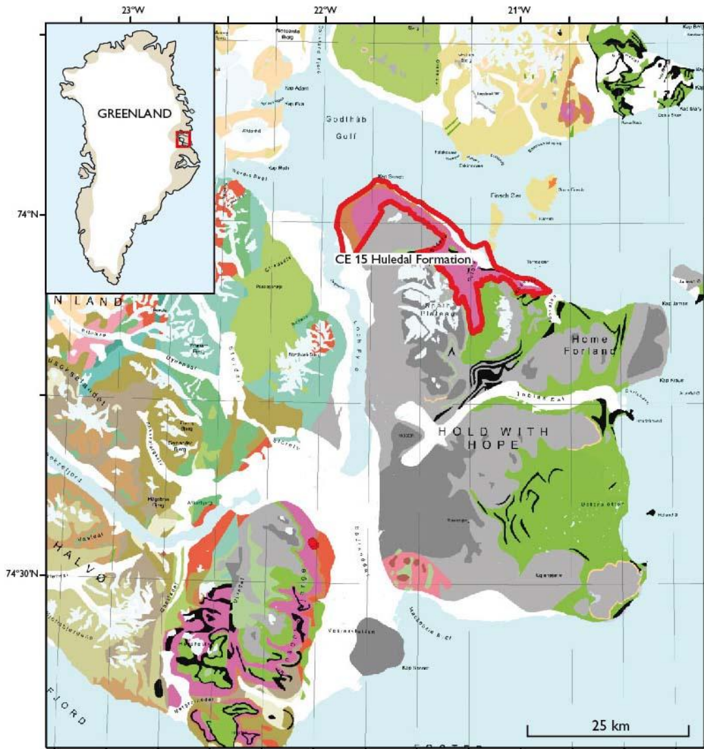
Figure 23. Outline of the Permian tract CE 15 Huledal Formation, Hold With Hope. The Huledal Formation, is shown in brown; Triassic units are shown in pink. See Appendix B for a geological legend.
