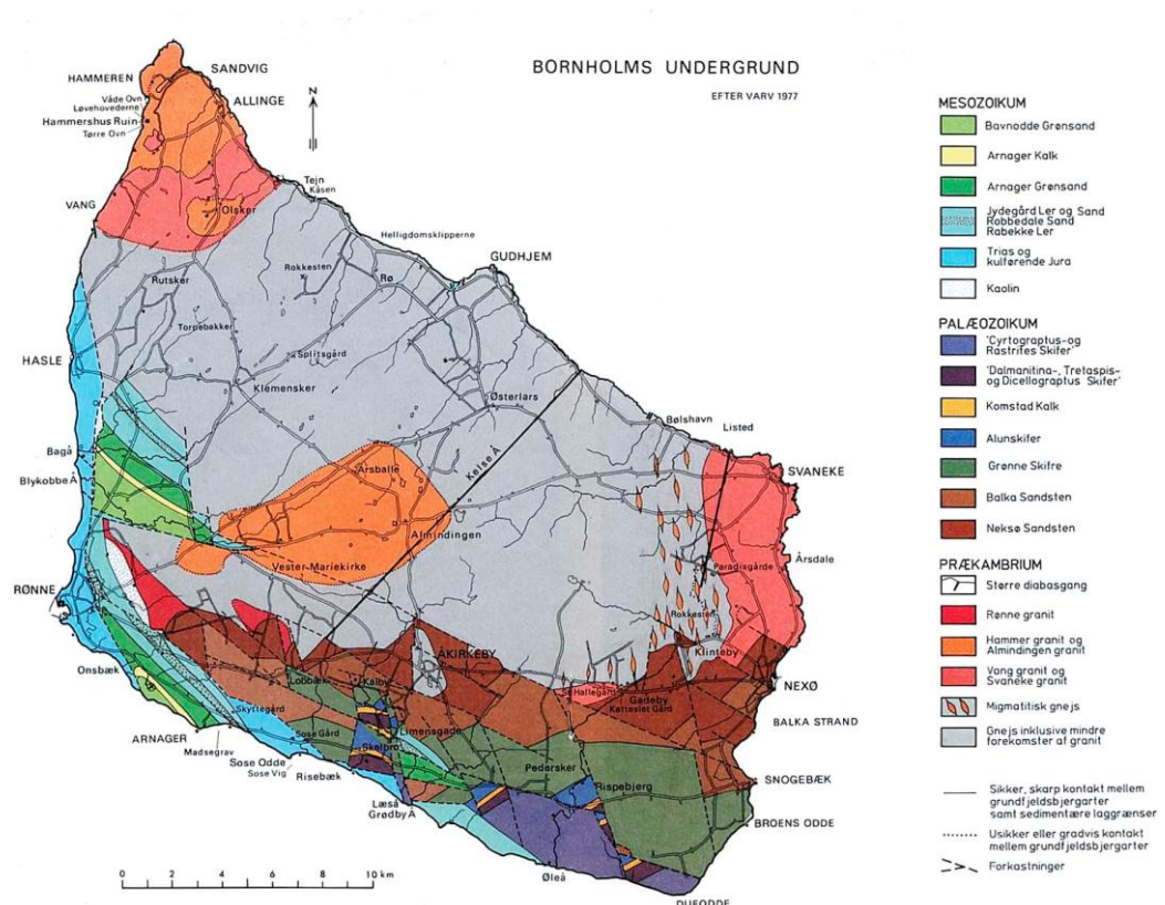
Figure 4. Map of the pre-Quaternary deposits and rocks of Bornholm (From VARV, 1977). Legend: Prækambrium: Precambrian (grey and red colours), Palæozoikum: Palaeozoic, Mesozoikum: Mesozoic.
