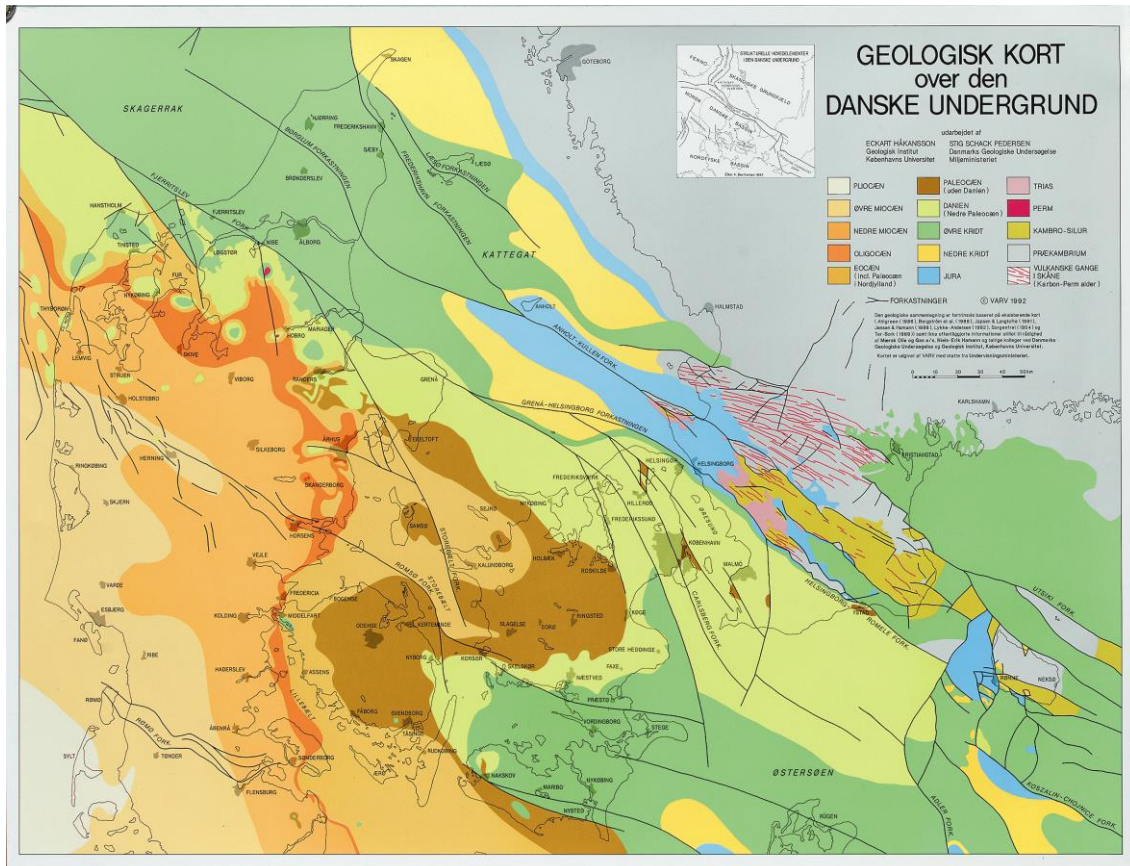
Figure 5. Map of the pre-Quaternary surface: Time units. Original scale: 1:50.000. Legend: Red lines: Precambrian intrusions. Grey: Precambrian. Olive: Cambrian-Silurian: Red: Permian. Light red: Triassic. Blue: Jurassic. Yellow: Lower Cretaceous. Green: Upper Cretaceous. Light green: Danian. Brown: Paleocene. Yellow olive: Eocene. Red brown: Oligocene. Light yellow brown: Lower Miocene. Very light yellow brown: Upper Miocene. White: Pliocene (Håkansson & Pedersen, 1992).
