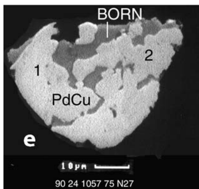
Back scatter images of selected Skaergaard minerals. c–d: skaergaardite (PdCu) in a sulphide droplet; e–f: free intergrowths of various noble metals minerals.
