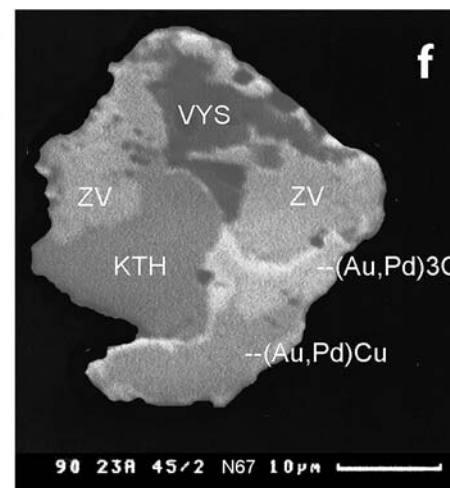
Back scatter images of selected Skaergaard minerals. c–d: skaergaardite (PdCu) in a sulphide droplet; e–f: free intergrowths of various noble metals minerals.
