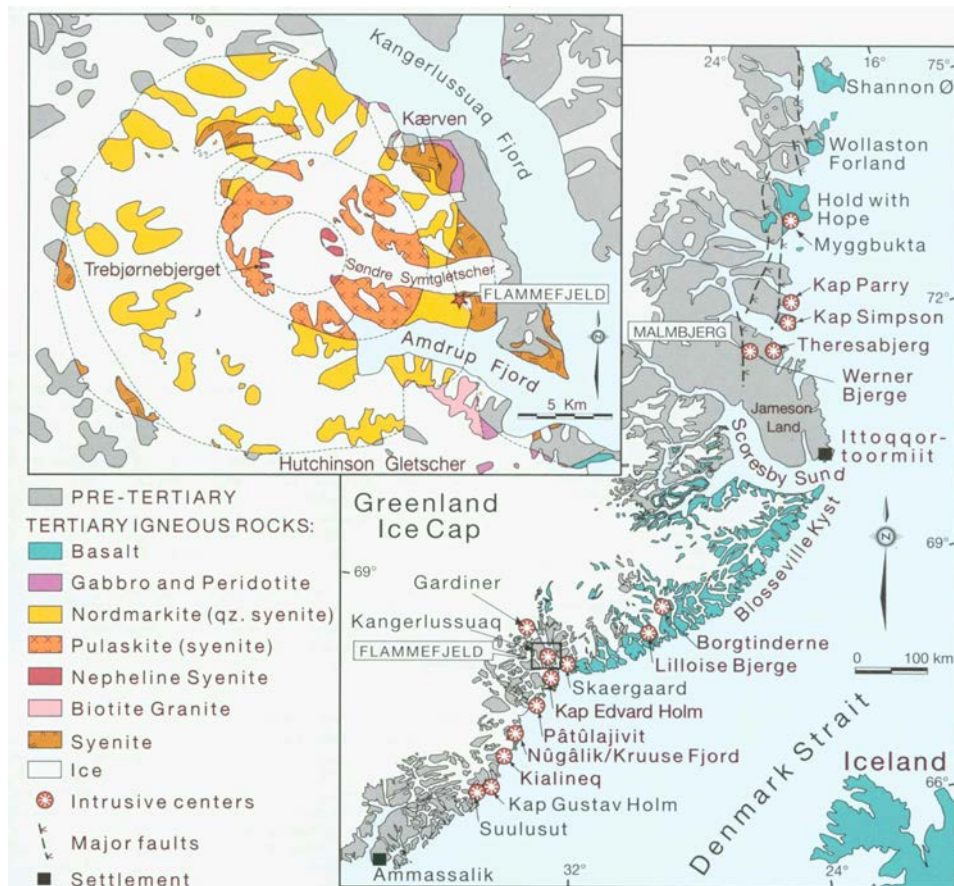
Figure 56. Distribution of Palaeogene igneous rocks in East Greenland. From Brooks et al. (2004).
