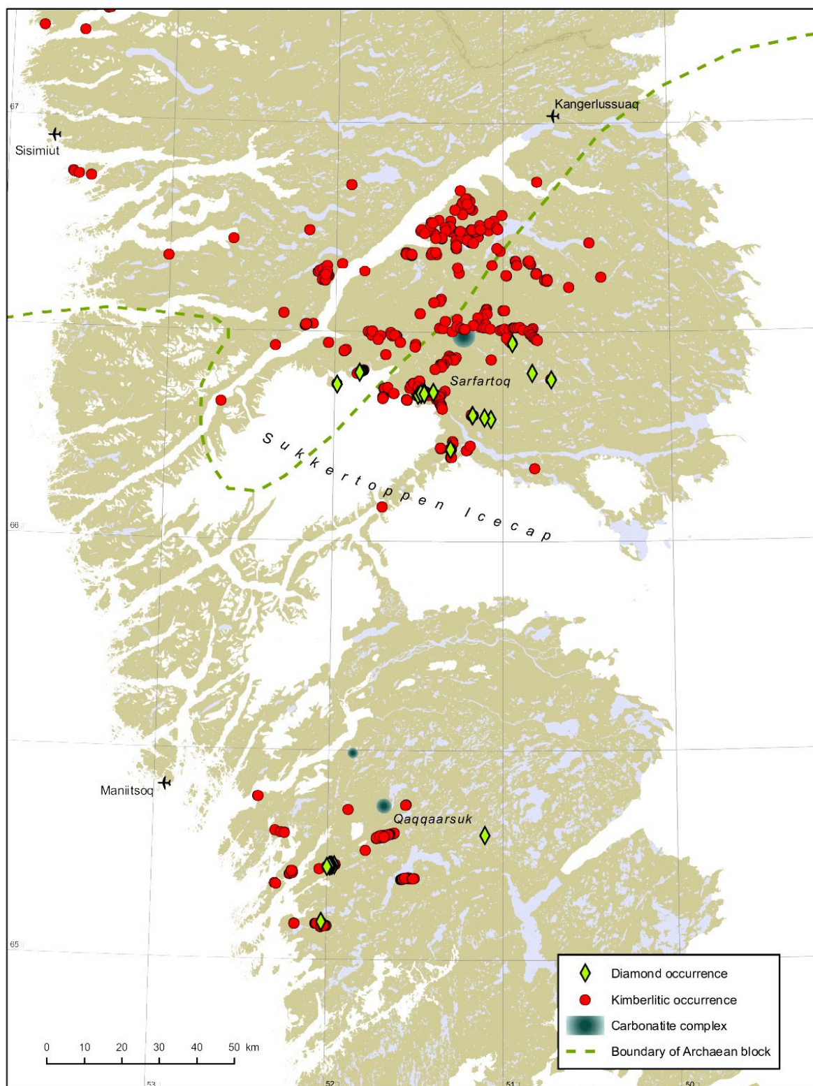
Figure 70. Map of kimberlitic and diamond occurrences in the Kangerlussuaq – anitsoq region, West Greenland.
